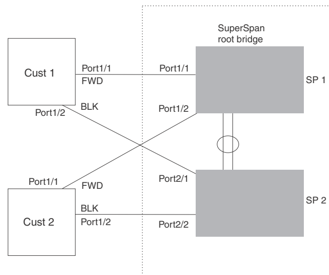
FIGURE 88 SuperSpan example
