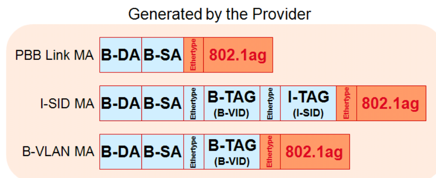
FIGURE 55 PBB MA Frames
