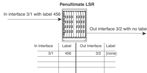
FIGURE 6 Penultimate hop popping
