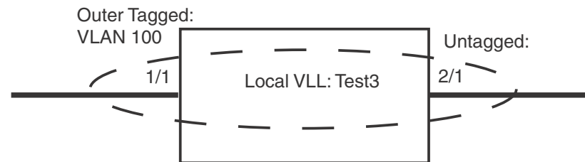
FIGURE 51 Local VLL “Test3” with 1 tagged VLAN and 1 untagged port
