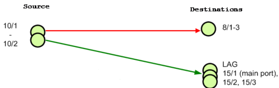
FIGURE 240 Configuration example 1
