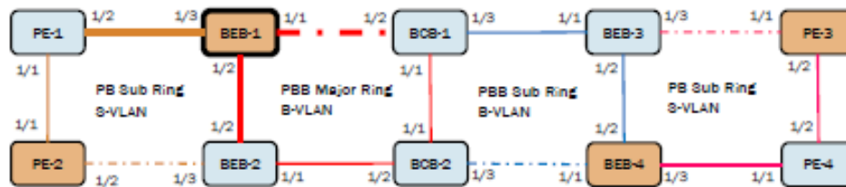
FIGURE 179 PBB interconnection node (BEB) sample configuration
