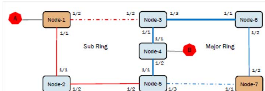
FIGURE 185 RAPS-propagate-tc
