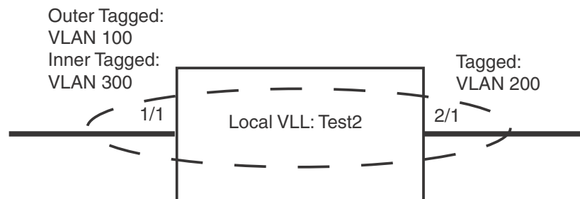
FIGURE 50 Local VLL “Test2” with 1 single-tagged VLAN and 1 dual-tagged VLAN
