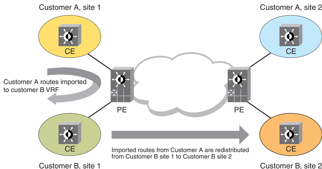
FIGURE 3 Inter-VRF routing topology
