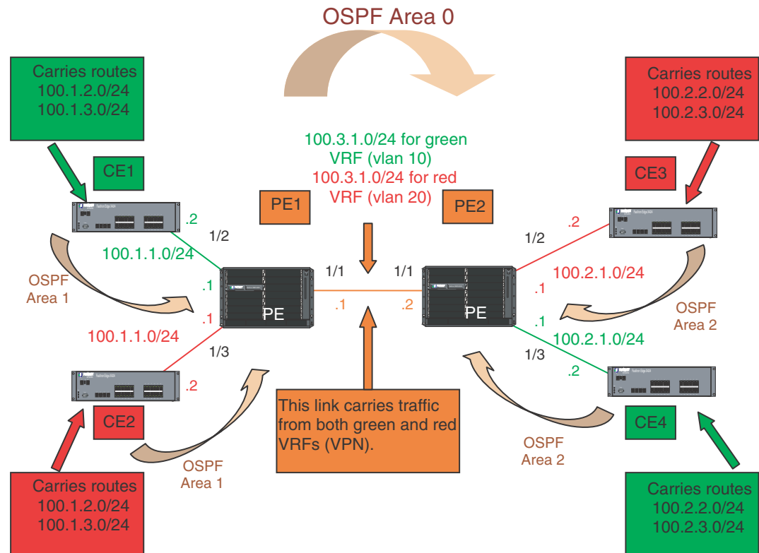
FIGURE 284 OSPF (Area 0) configured between PE1 and PE2 with OSPF (Area 1 and Area 2) configured between PEs and CEs
