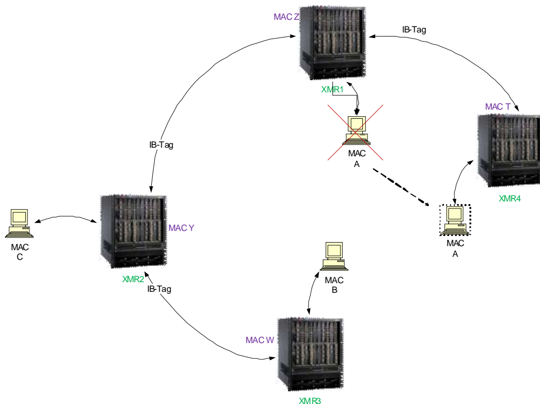
FIGURE 51 MAC Learning for PBB packets
