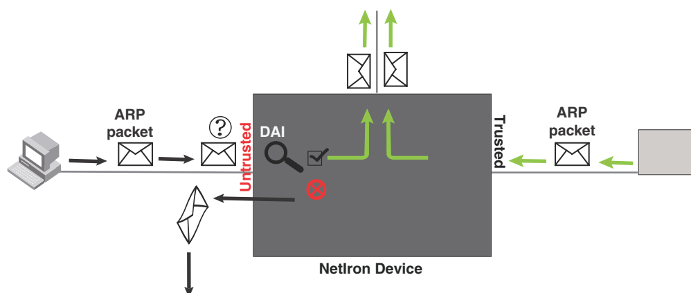
FIGURE 226 Dynamic ARP inspection at work
