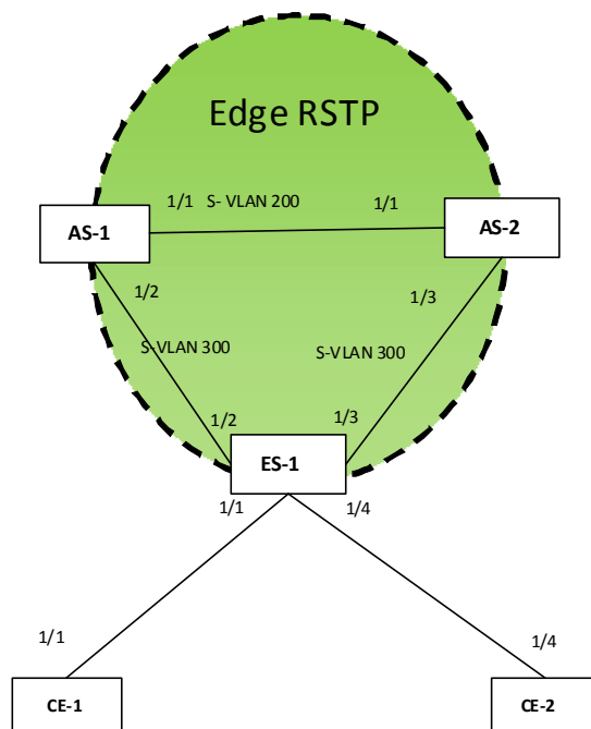
FIGURE 130 Edge RSTP topology 2
