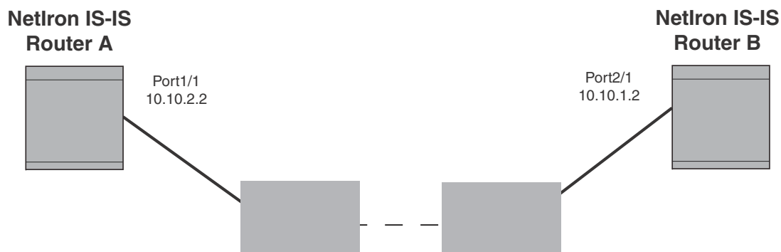
FIGURE 255 IS-IS Point-to-Point configuration
