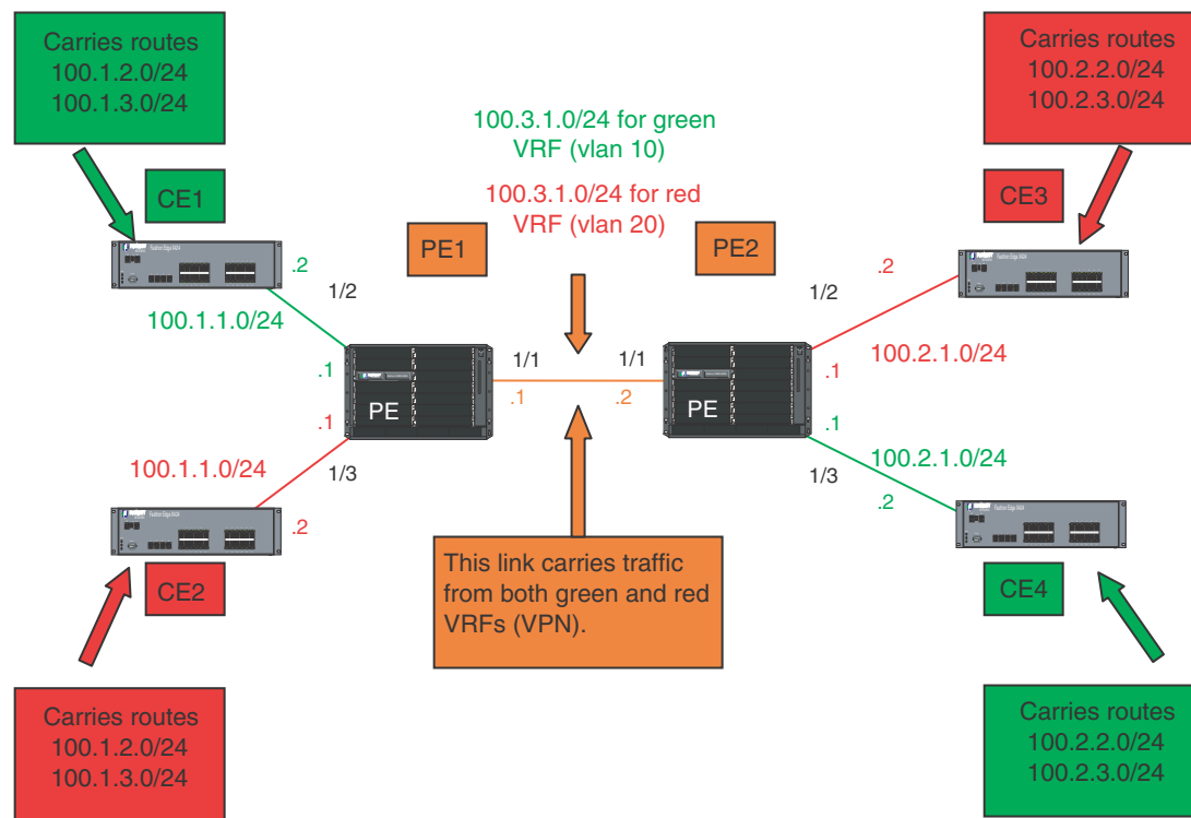
FIGURE 282 Example network topology with both RED and GREEN VPNs
