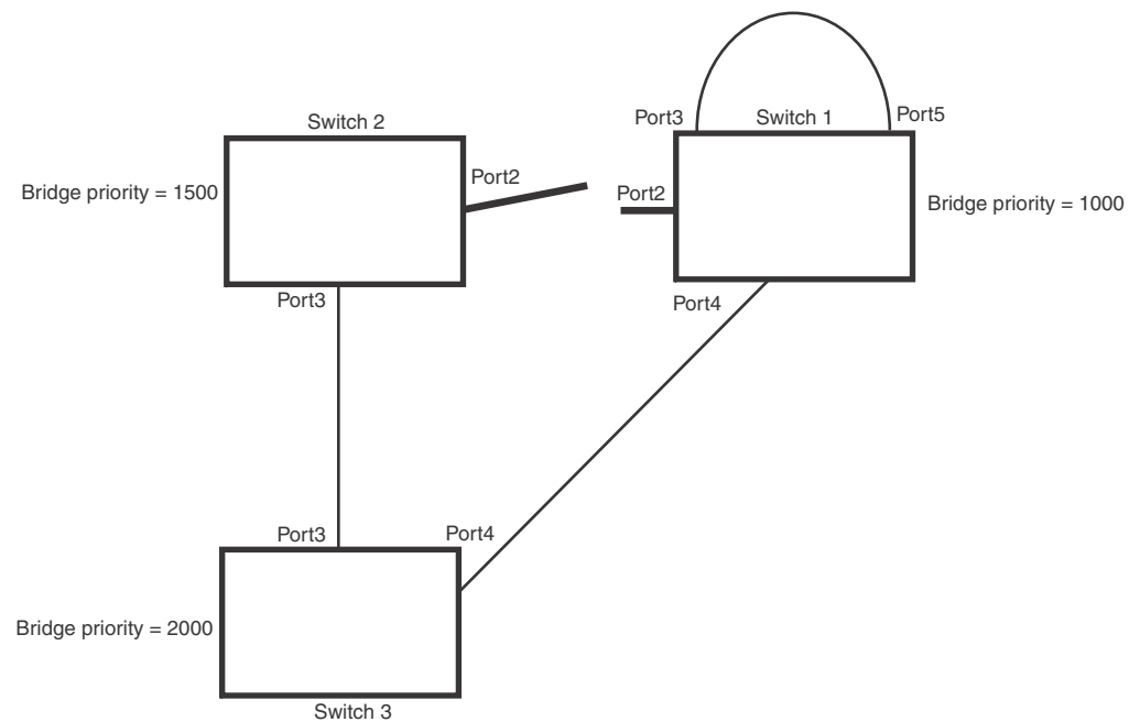
FIGURE 119 Link failure in the topology
