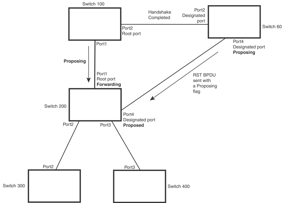
FIGURE 111 New root bridge sending a proposal flag
