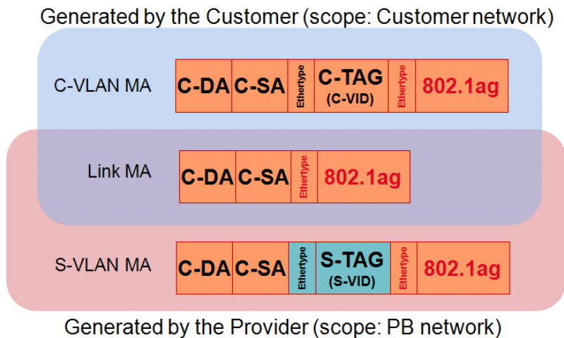
FIGURE 54 S-VLAN, C-VLAN, and Link MA Frames
