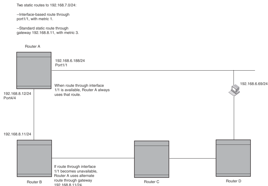
FIGURE 234 Standard and interface routes to the same destination network
