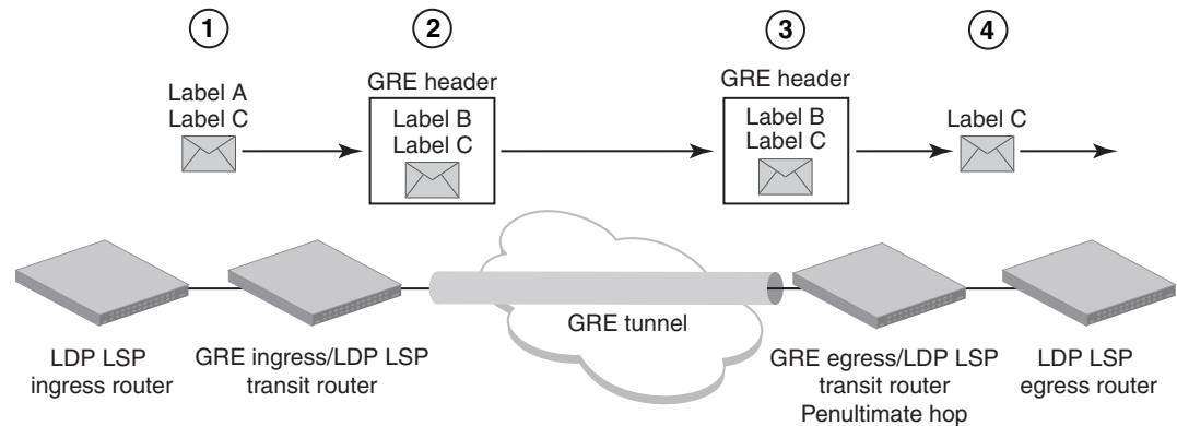
FIGURE 42 LDP VPLS over a GRE tunnel example
