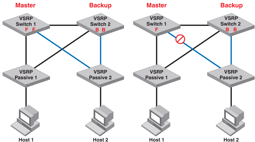
FIGURE 195 Black hole scenario 2
