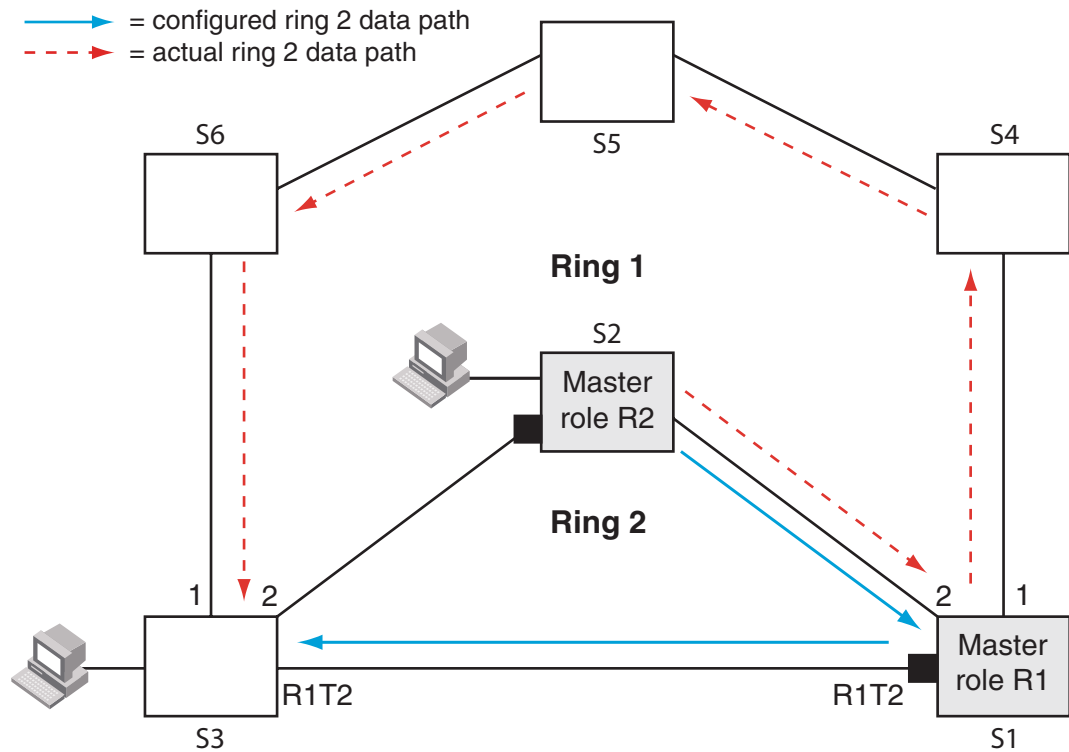
FIGURE 150 Unexpected switching path with shared interface
