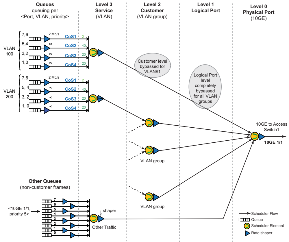
FIGURE 72 Bypassing hierarchy levels example
