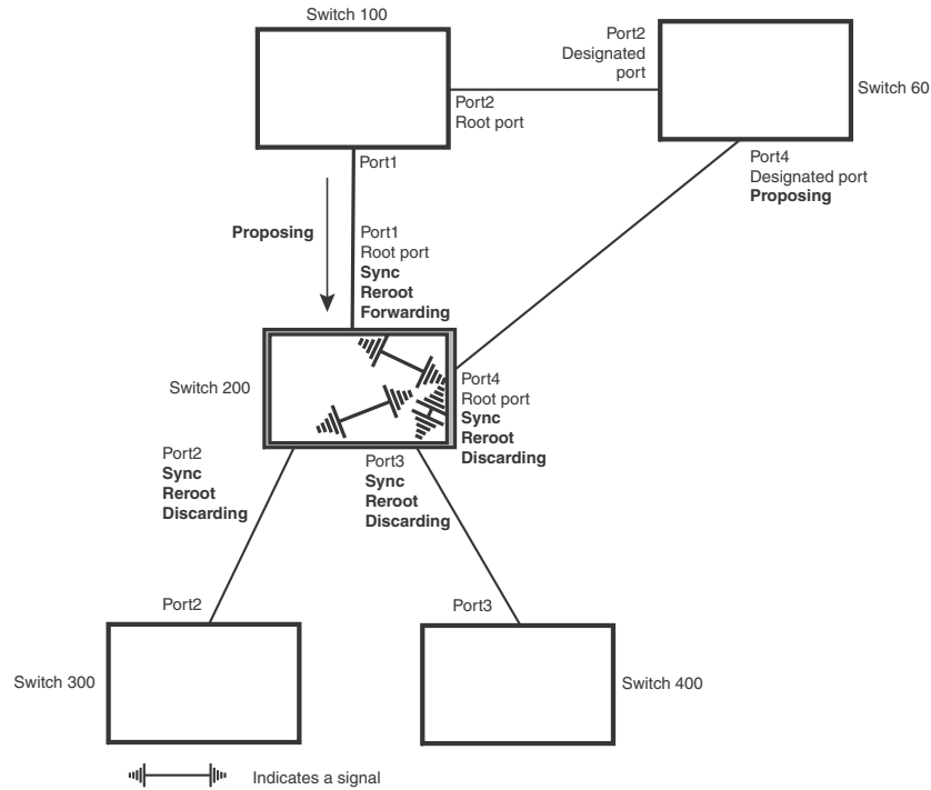
FIGURE 112 Sync and reroot
