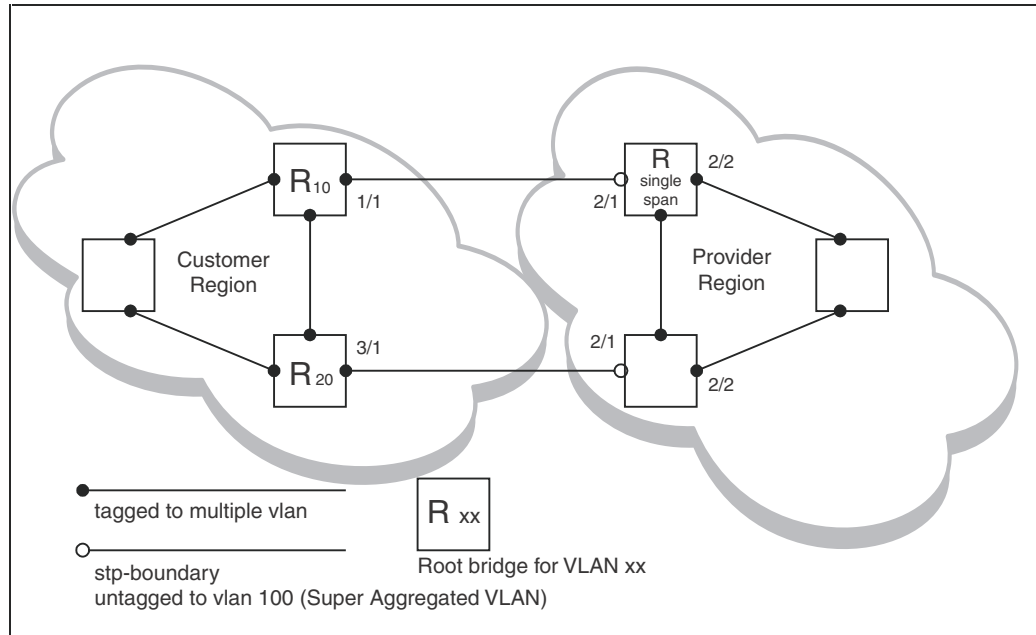
FIGURE 92 Customer using Single STP and SP using multiple spanning trees
