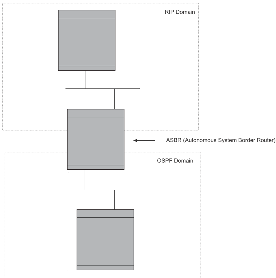
FIGURE 249 Redistributing OSPF and static routes to RIP routes
