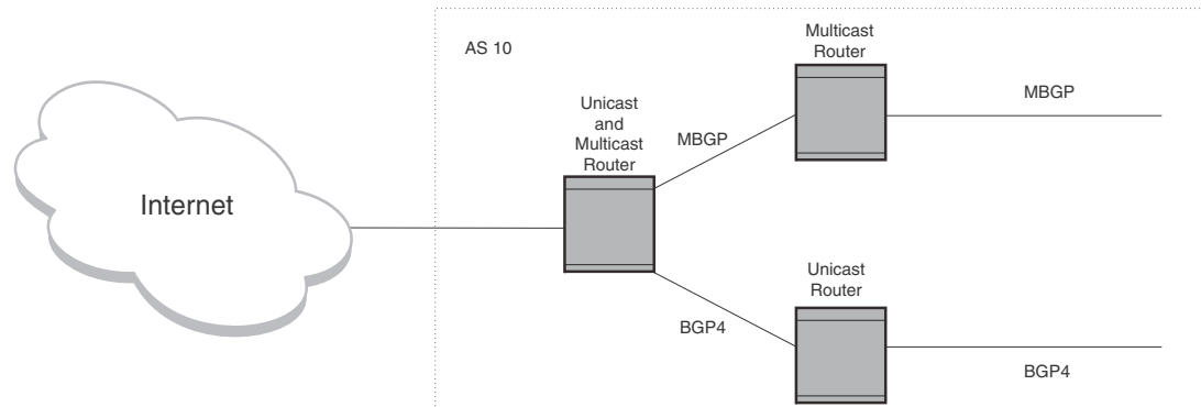
FIGURE 278 MBGP used when multicast topology is different from unicast topology
