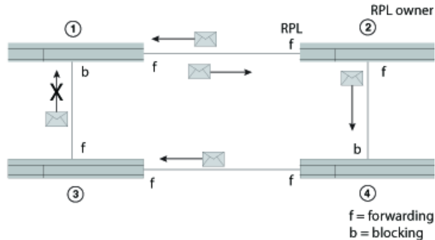
FIGURE 161 Initializing an ERP topology - III
