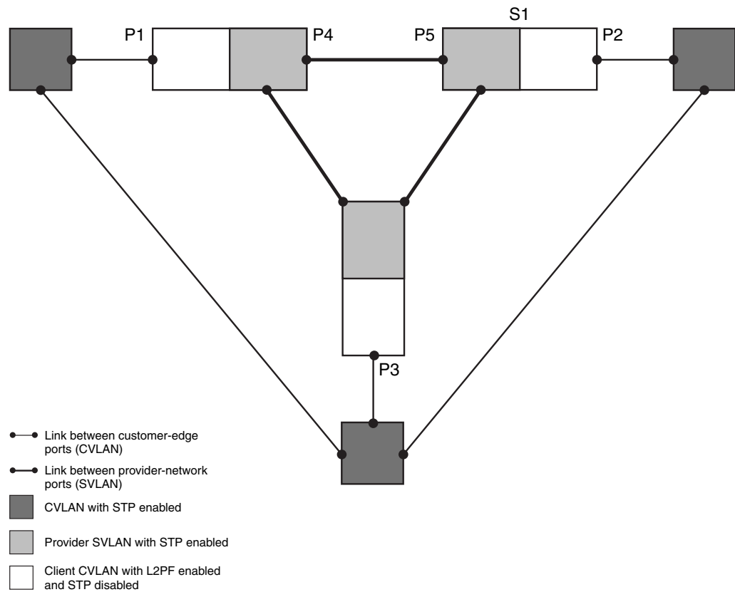
FIGURE 29 L2PF in a network
