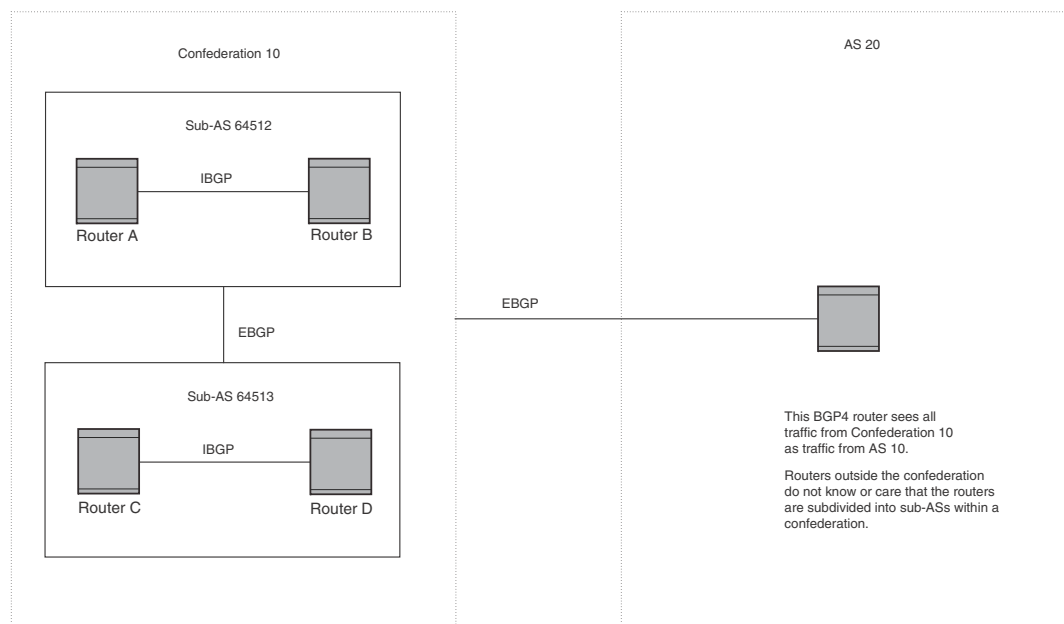
FIGURE 262 Example BGP4 confederation
