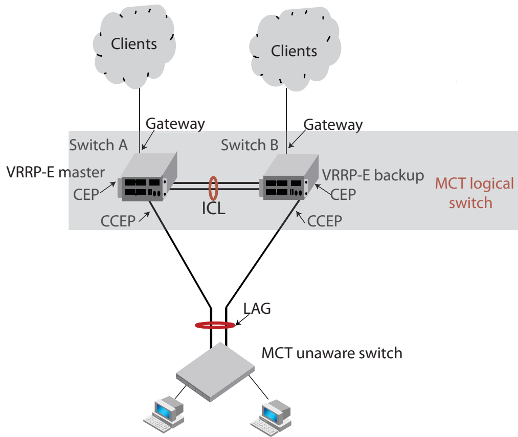
FIGURE 214 Example of MCTS that are Layer 2 switched
