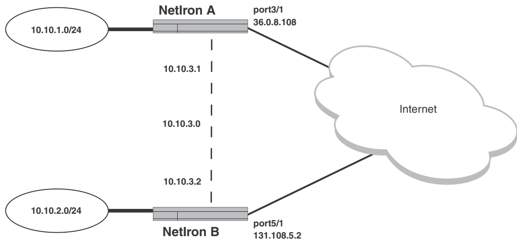
FIGURE 222 GRE IP tunnel configuration example
