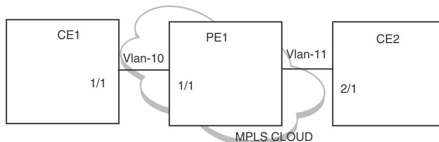
FIGURE 110 IEEE 802.1ag over VLL-LOCAL
