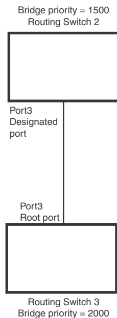
FIGURE 116 Convergence between two bridges
