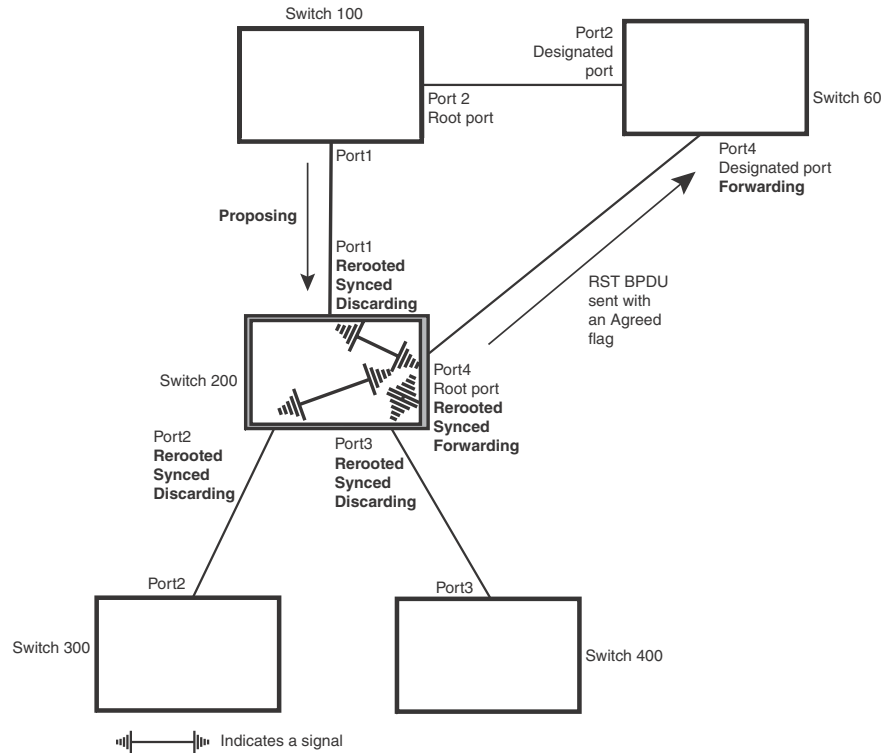
FIGURE 114 Rerouted, synced, and agreed
