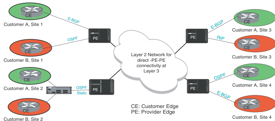
FIGURE 281 Multi-VRF in a service provider application
