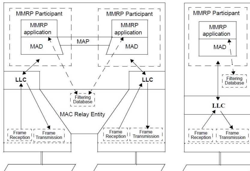
FIGURE 95 MMRP components
