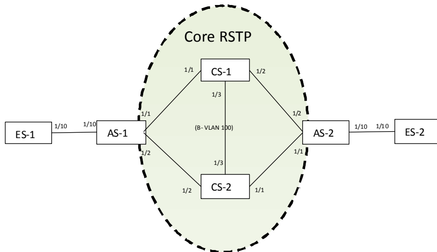
FIGURE 134 Core RSTP inPBB network
