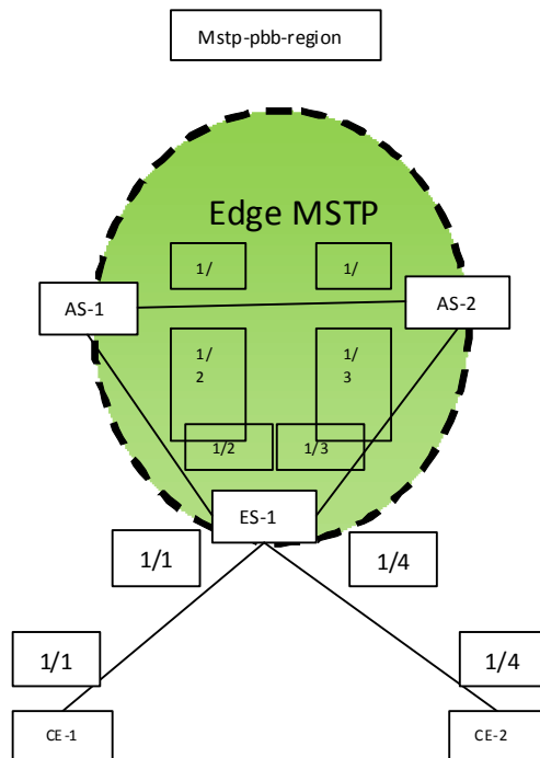
FIGURE 101 Edge MSTP in a PB network
