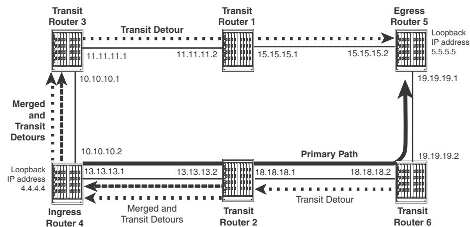
FIGURE 36 MPLS Fast Reroute Loop configuration
