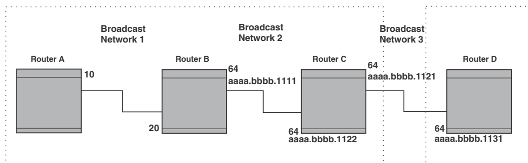
FIGURE 253 Each broadcast network has a Level-1 Designated IS and a Level-2 Designated IS
