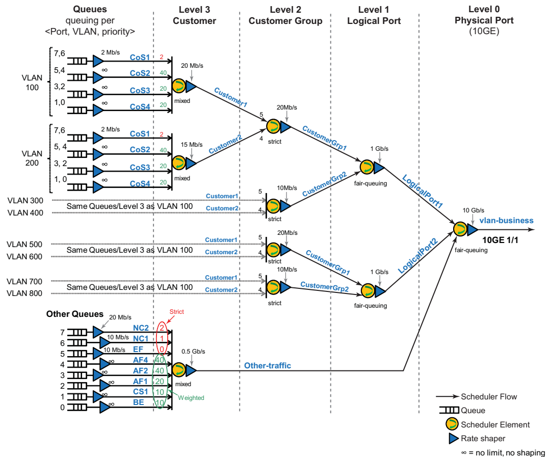
FIGURE 73 Other traffic example
