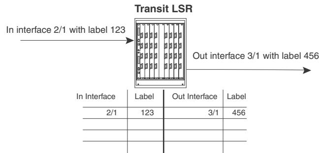
FIGURE 5 Label swapping on a transit LSR
