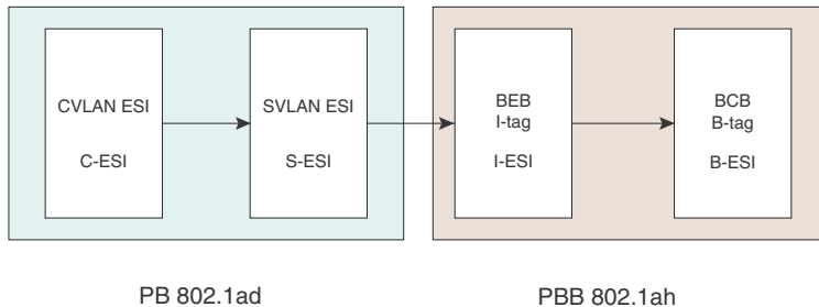
FIGURE 40 Association of ESI and VLAN for different stages
