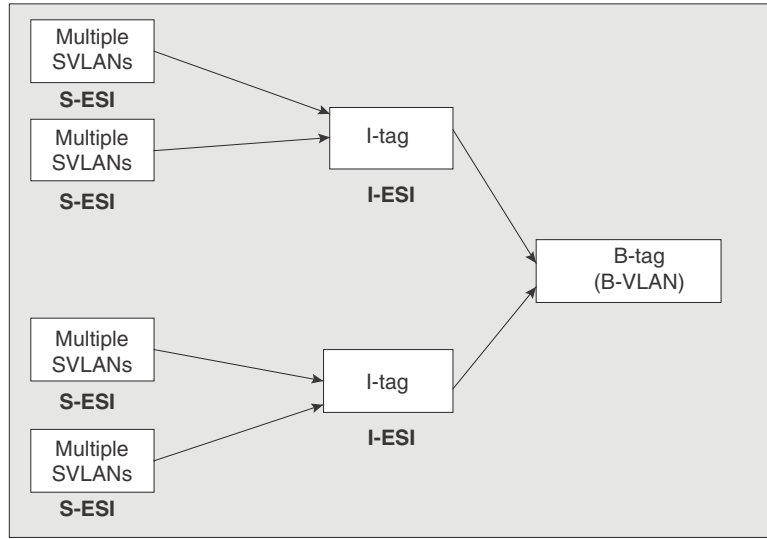
802.1ah PBB: I-tags belonging to a B-tag need to be unique
