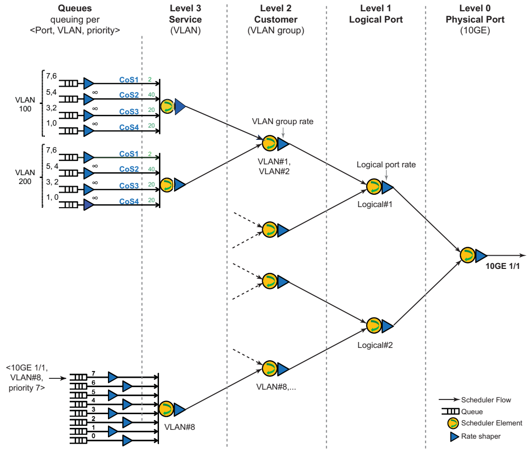
FIGURE 75 HQoS for Local VPLS model
