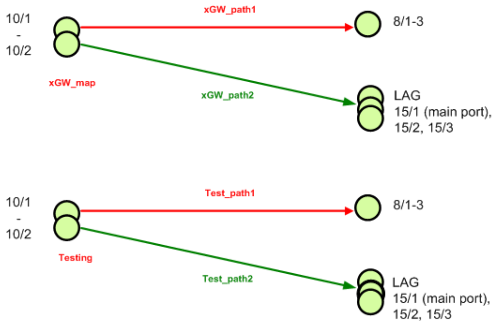
FIGURE 241 Configuration example 2
