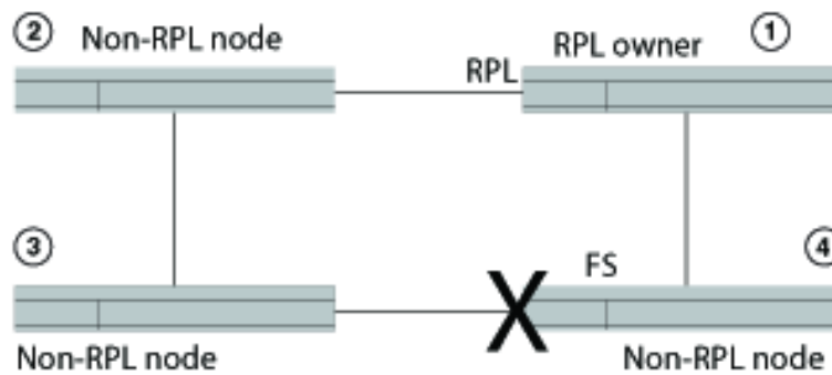
FIGURE 171 Single forced switch scenario
