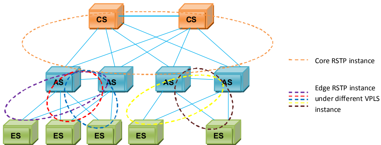
FIGURE 126 RSTP isolation in dual homing of AS and ES
