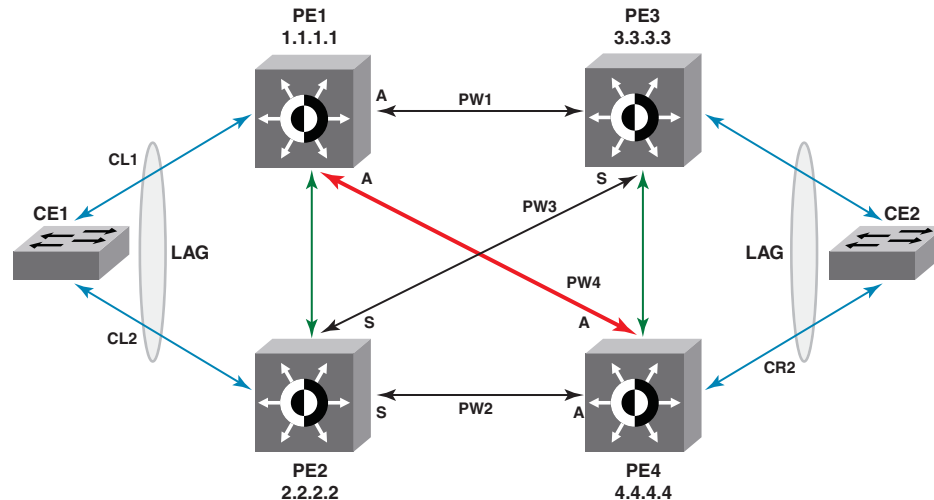
FIGURE 217 Sample topology with MCT end-points for VLL
