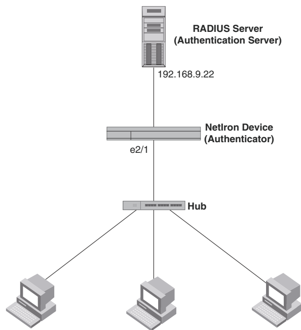
FIGURE 100 Multiple clients connected to a single 802.1x-enabled port
