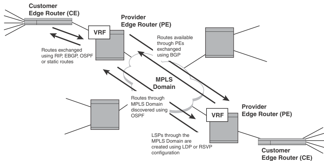
FIGURE 60 BGP or MPLS VPN route discovery
