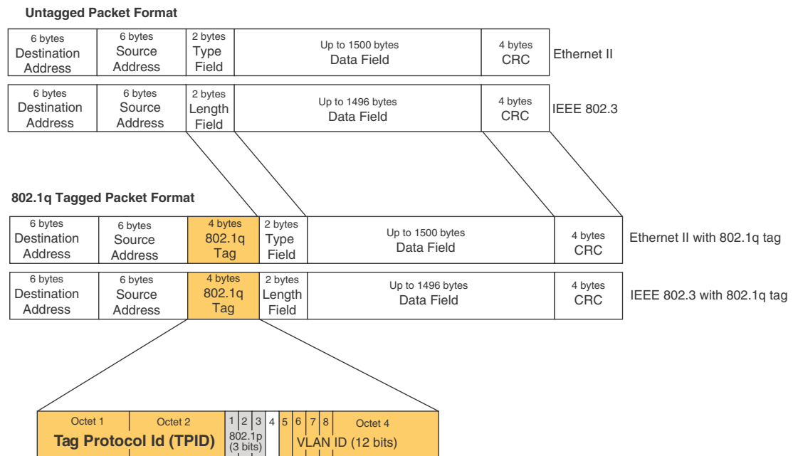
FIGURE 10 Packet containing Brocade's 802.1QVLAN tag
