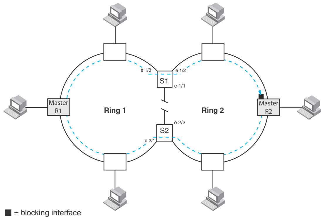
FIGURE 154 Flow of RHP packets when a link for shared interfaces breaks
