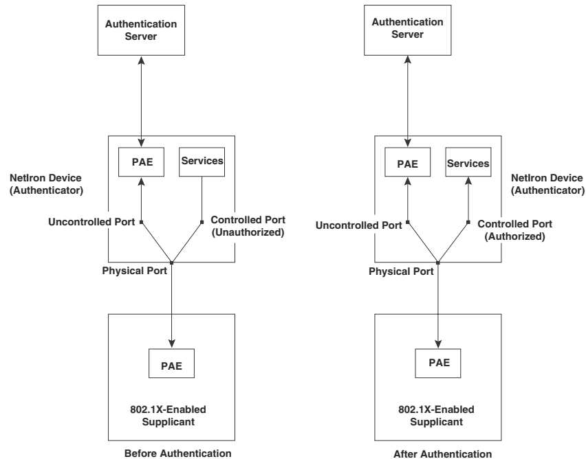
FIGURE 98 Controlled and uncontrolled ports before and after client authentication
