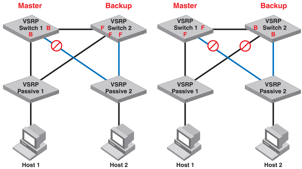
FIGURE 196 Black hole scenario 3
