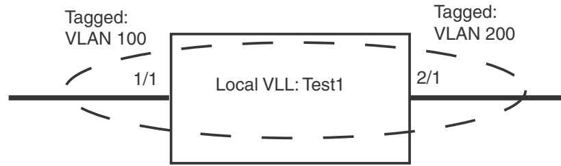
FIGURE 49 Local VLL “Test1” with 2 tagged VLANs
