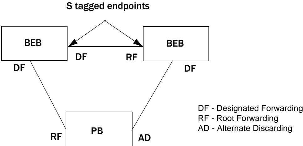
FIGURE 127 RSTP convergence when two AS connected via S tagged endpoint
