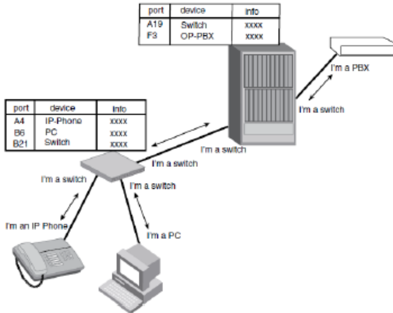
FIGURE 4 LLDP connectivity
