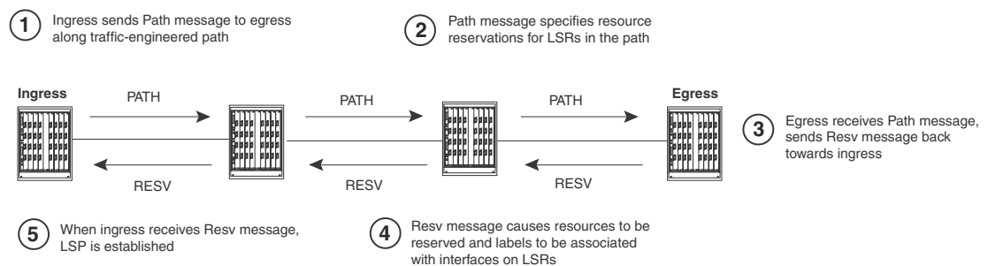
FIGURE 9 How RSVP establishes a signalled LSP
