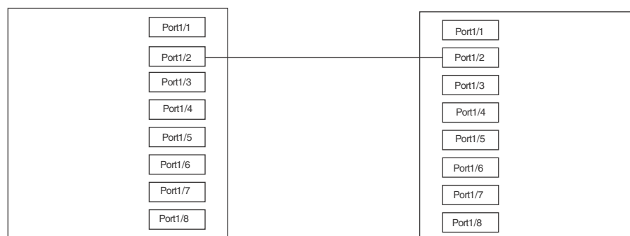
FIGURE 5 Example of a 1-port keep alive LAG
