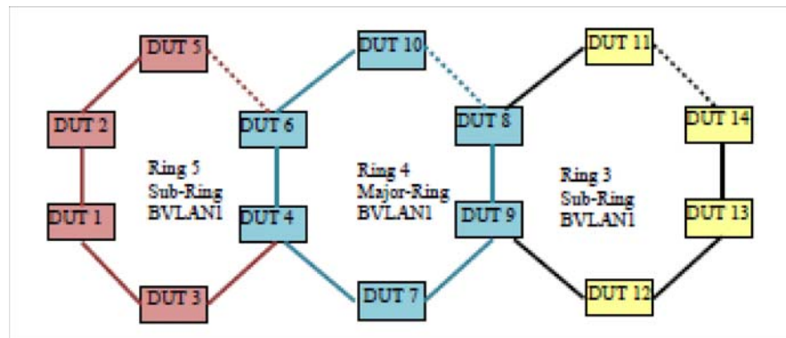
FIGURE 177 ERP configuration with same VLAN
