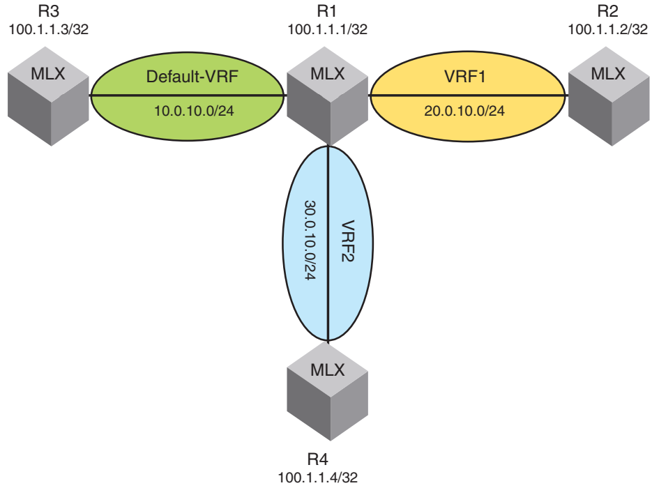
FIGURE 1 A Network deploying Inter-VRF
