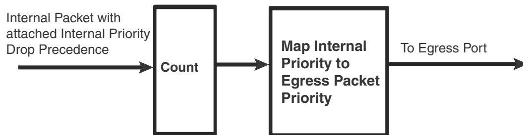
FIGURE 60 Logic flow of Egress QoS processing
