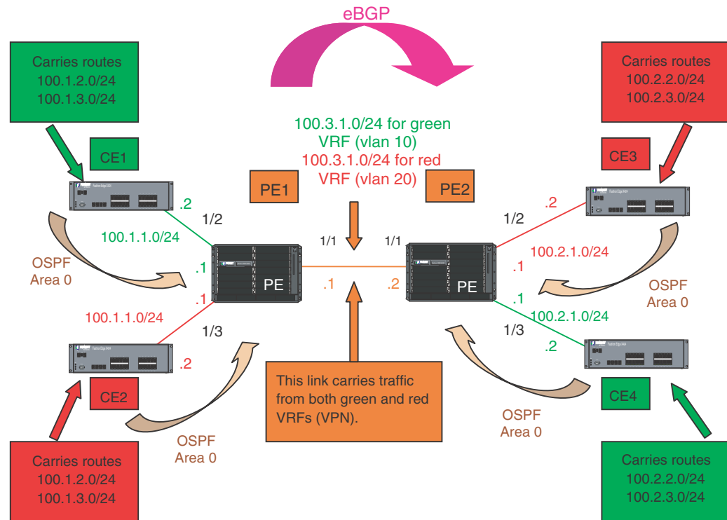
FIGURE 283 eBGP configured between PE1 and PE2 with OSPF (Area 0) configured between PEs and CEs
