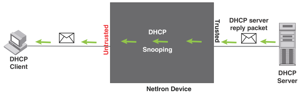
FIGURE 228 DHCP snooping at work - on trusted port
