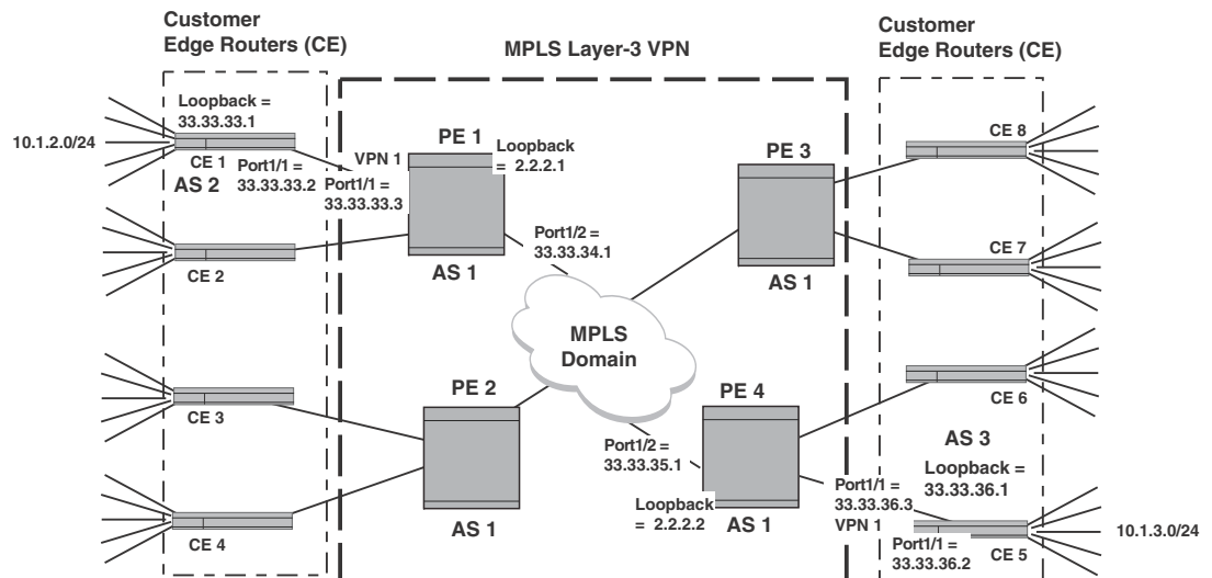
FIGURE 63 EBGP to CE network example
