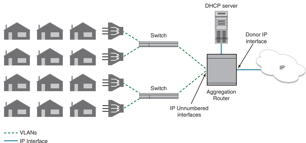
FIGURE 224 IP Unnumbered Interfaces feature
