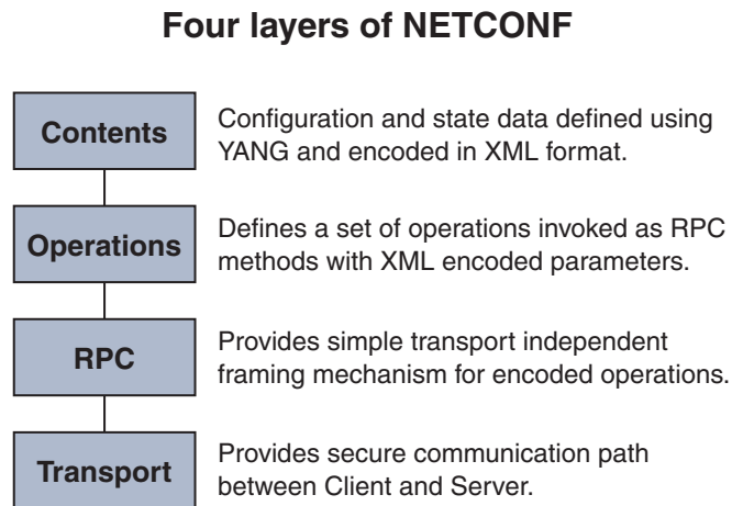
FIGURE 116 Four layers of NETCONF
