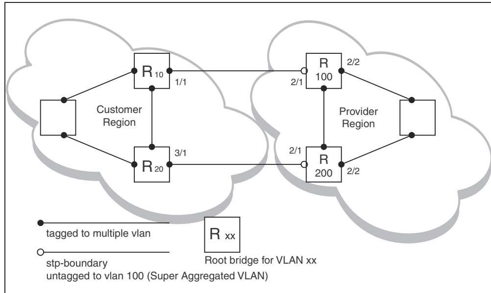
FIGURE 90 Customer and SP using multiple spanning trees
