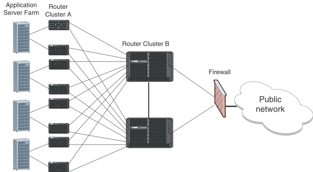
FIGURE 280 Example of Multi-VRF usage in an enterprise data center application
