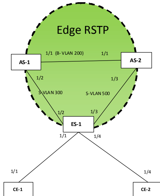
FIGURE 132 Edge RSTP topology 4
