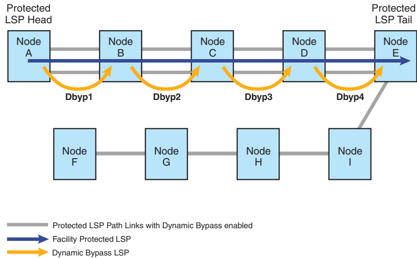
FIGURE 32 Dynamic bypass creation with link protection PLRs.c
