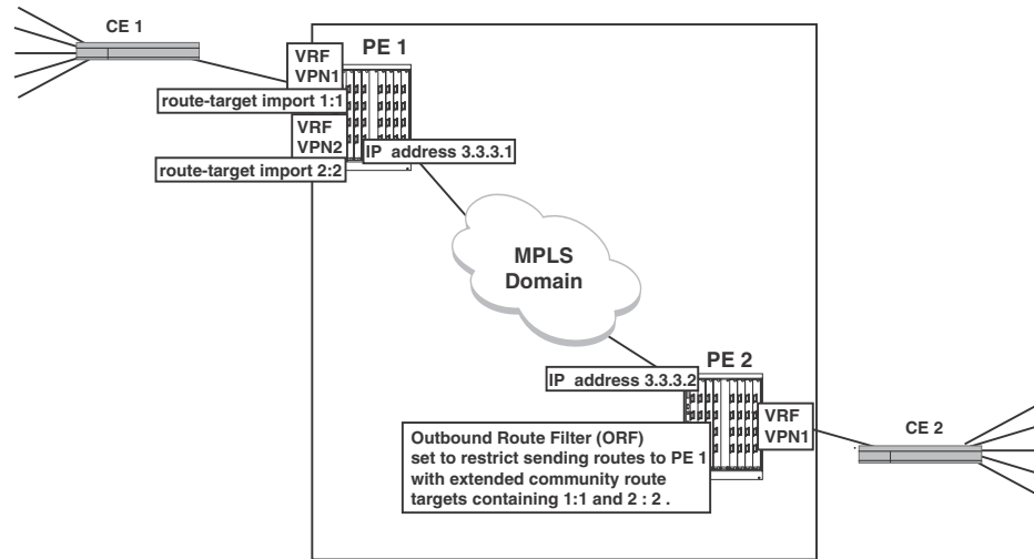
FIGURE 67 Cooperative route filtering example
