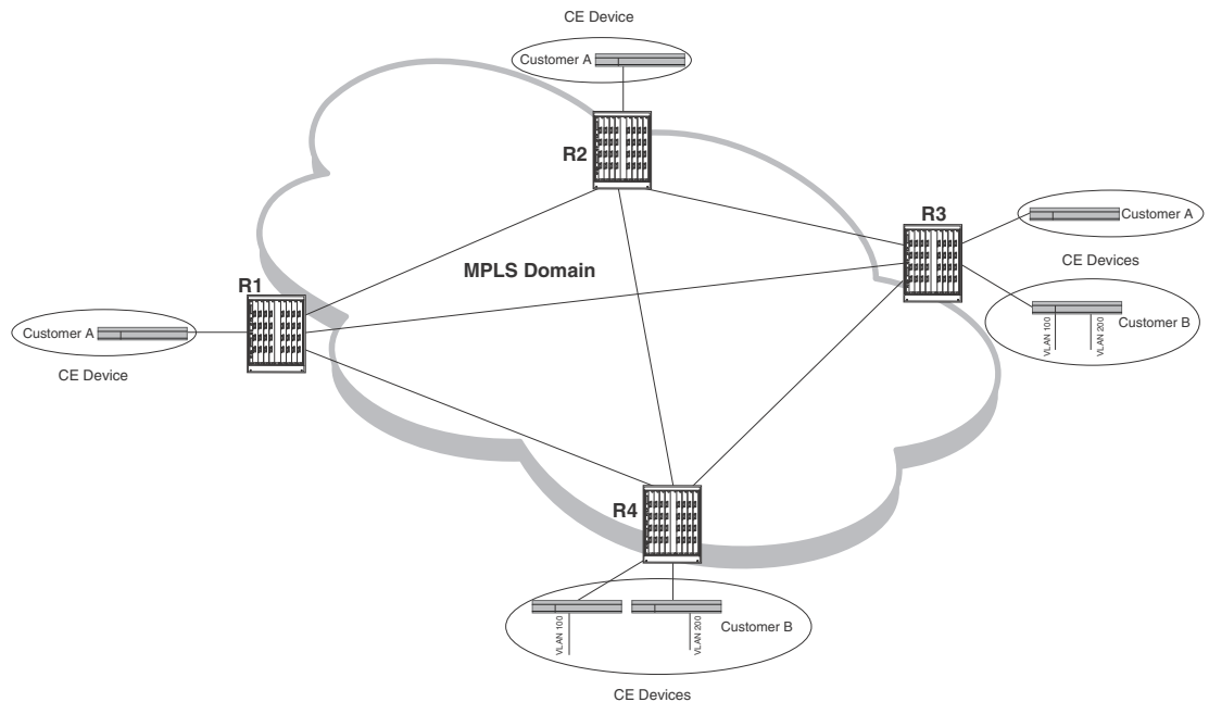
FIGURE 52 Sample VPLS configuration
