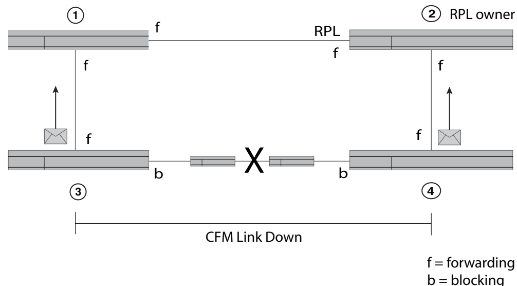
FIGURE 156 ERP with IEEE 802.1ag support
