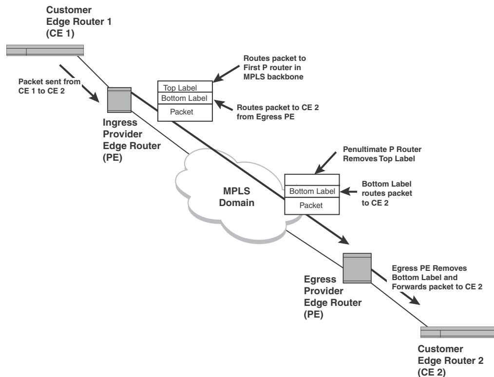
FIGURE 61 Routing a packet through a BGP or MPLS VPN
