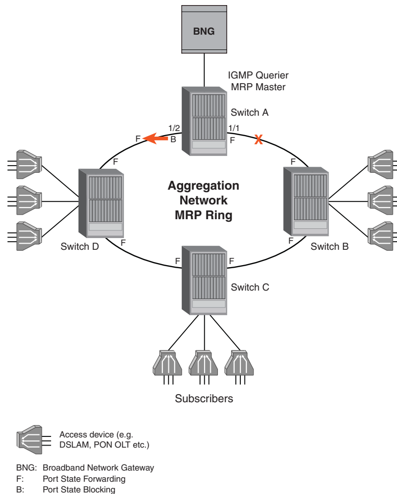
FIGURE 142 MRP ring with switch A as the querier
