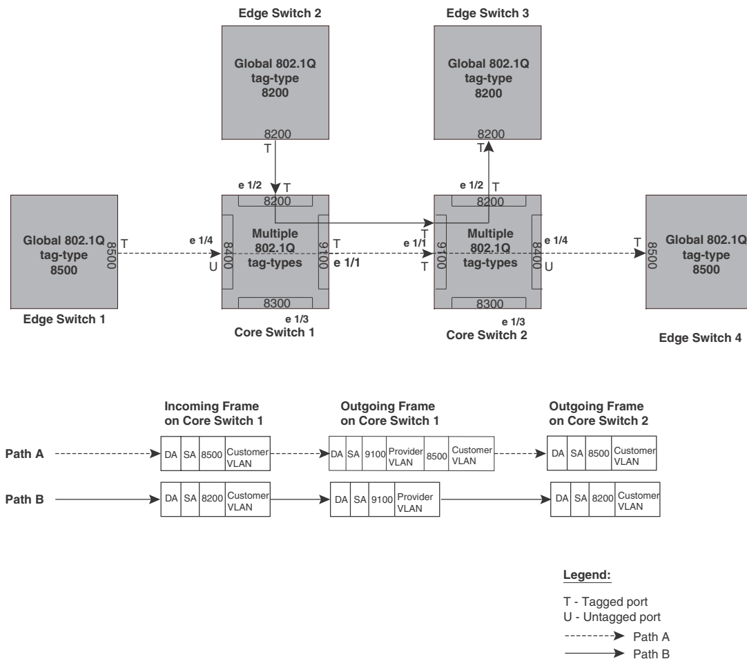
FIGURE 19 802.1q Tag-type translation configuration example 2
