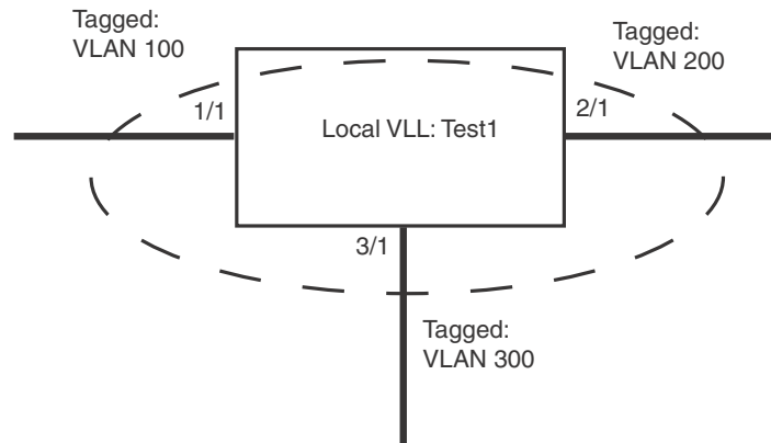
FIGURE 56 Local VPLS “Test1” with three tagged VLANs
