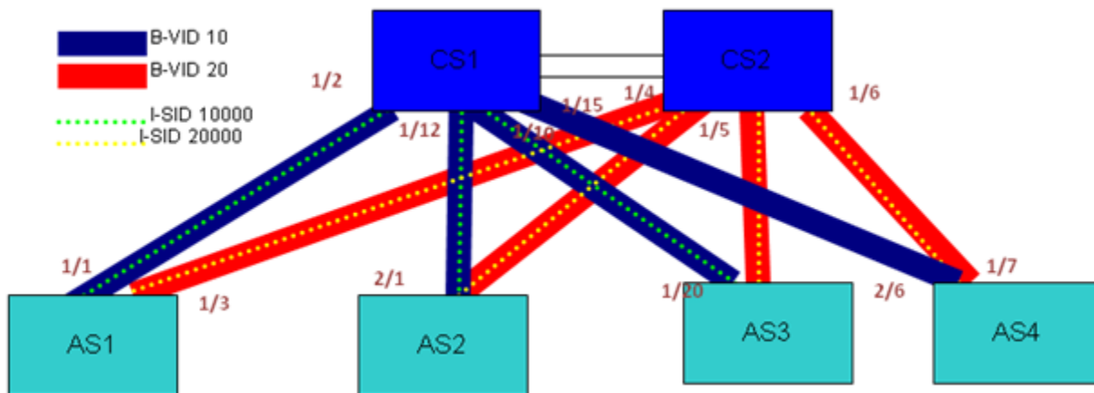
FIGURE 93 MMRP with PBB enabled
