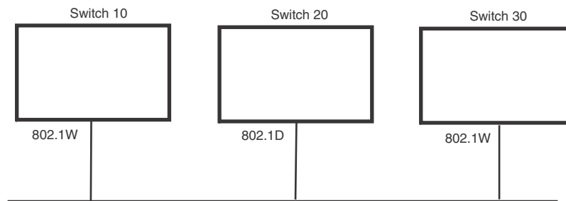
FIGURE 125 RSTP bridges with an 802.1D bridge
