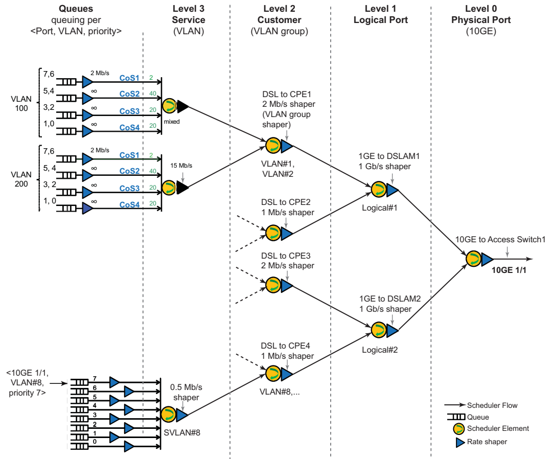
FIGURE 74 HQoS example
