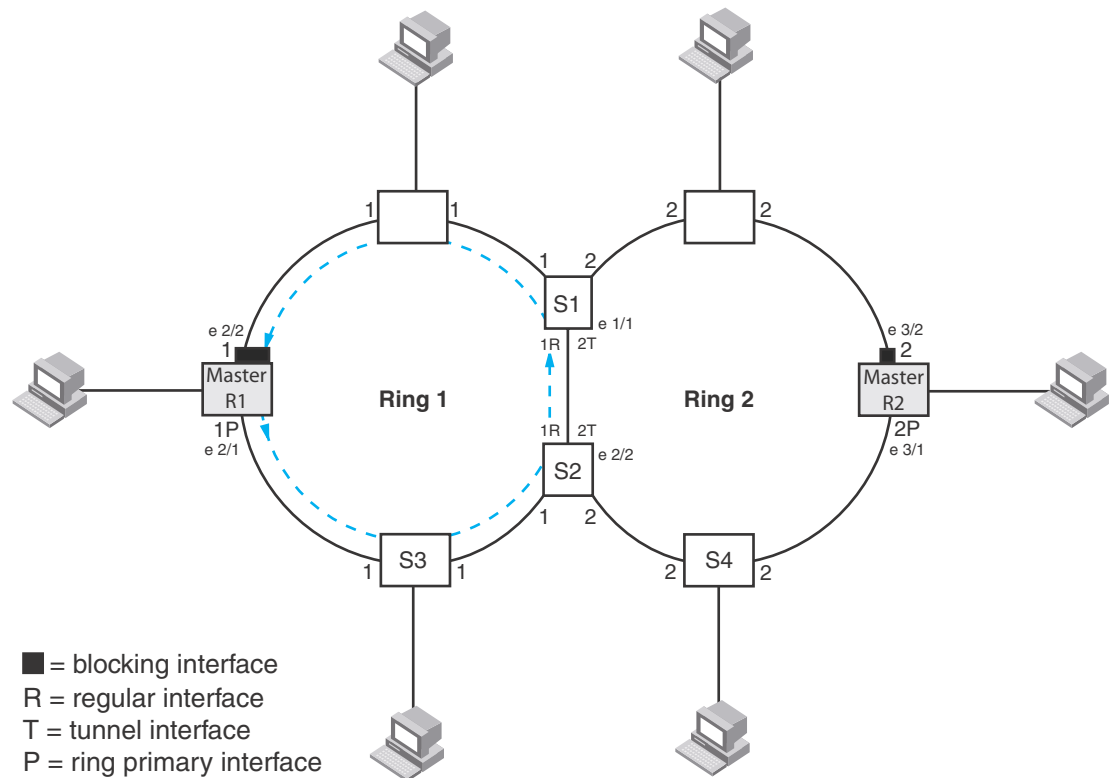
FIGURE 153 RHP flow on rings with shared interfaces showing ring 2 RHP flow
