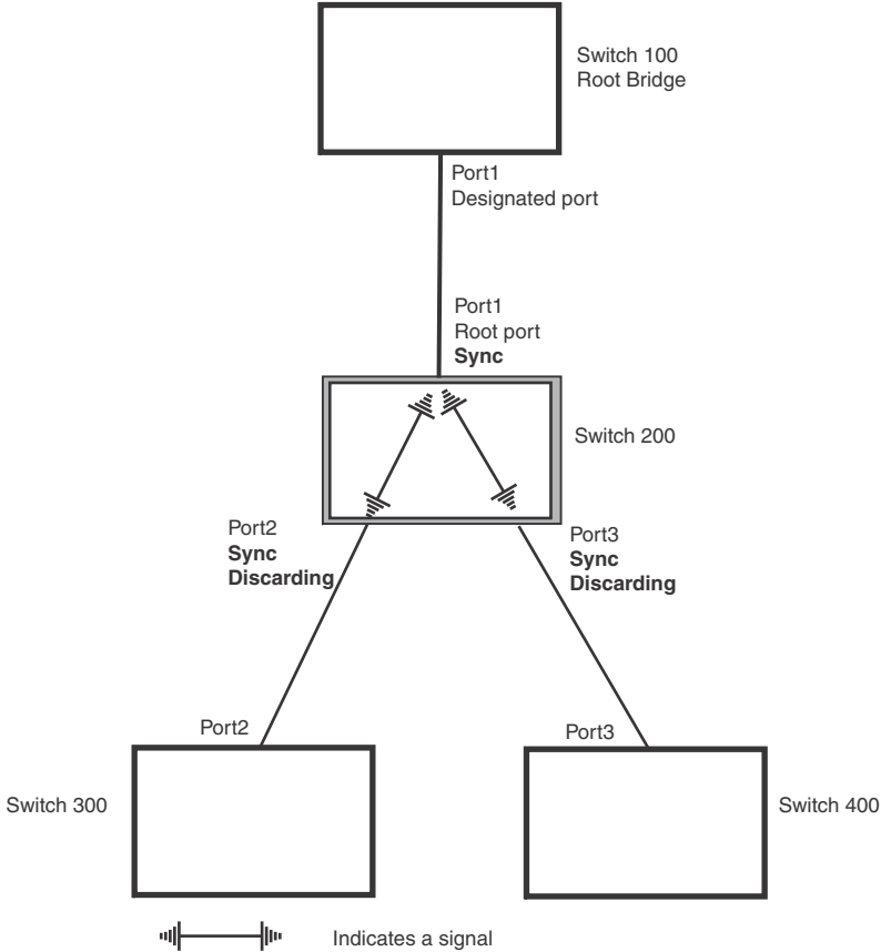
FIGURE 107 Sync stage
