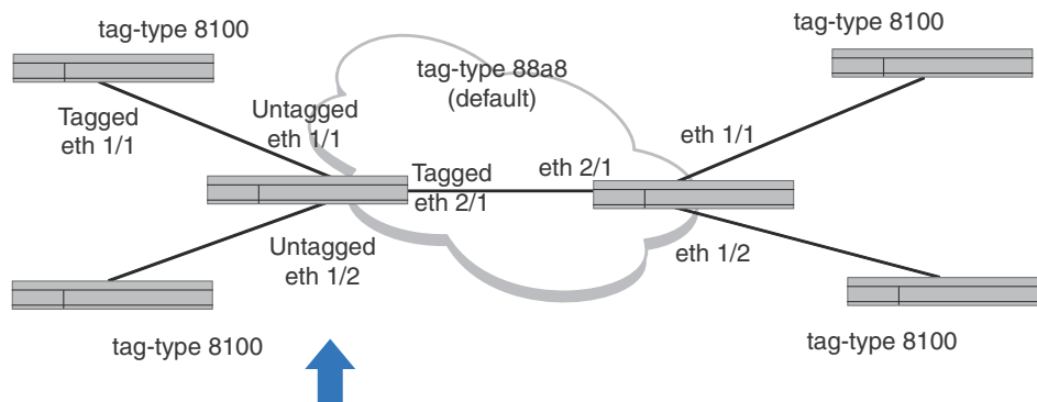
FIGURE 28 Port-based service interface
