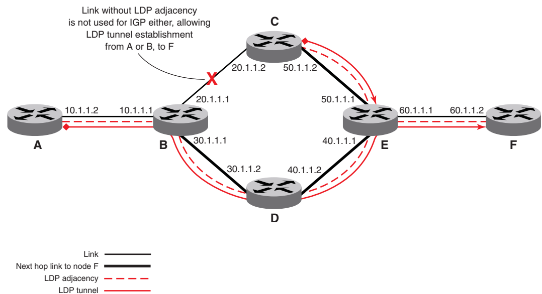
FIGURE 34 Example with LDP IGP synchronization
