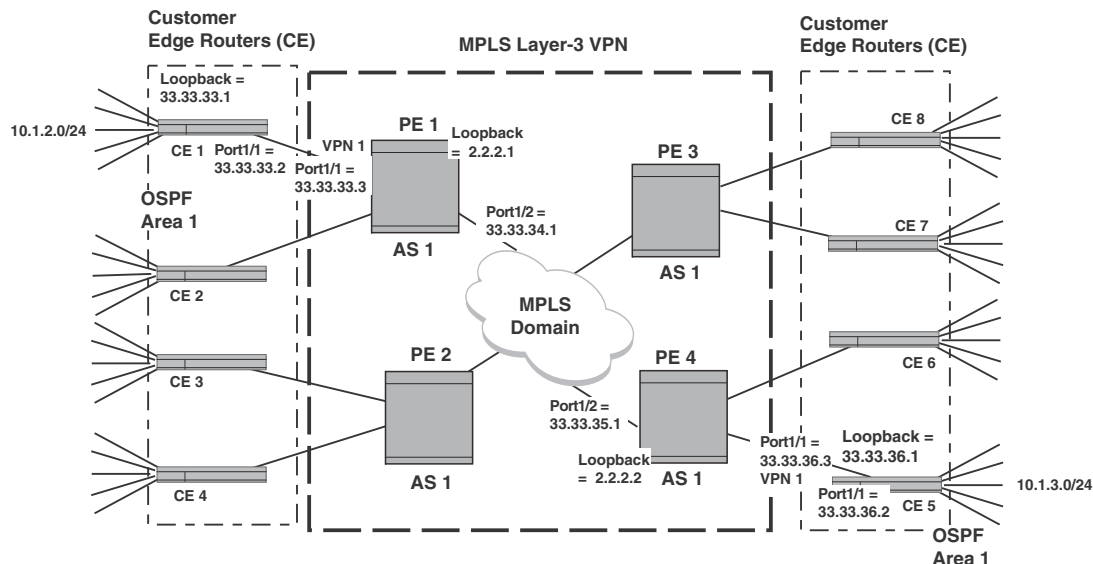
FIGURE 66 OSPF to CE network example
