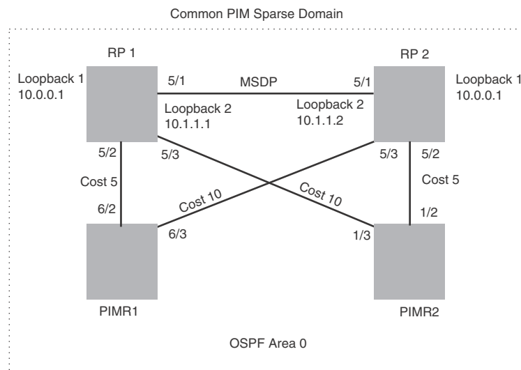
FIGURE 270 Example of a MDSP Anycast RP network
