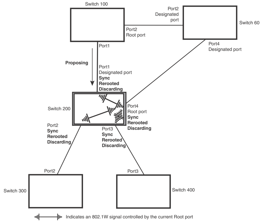
FIGURE 113 Sync and rerooted
