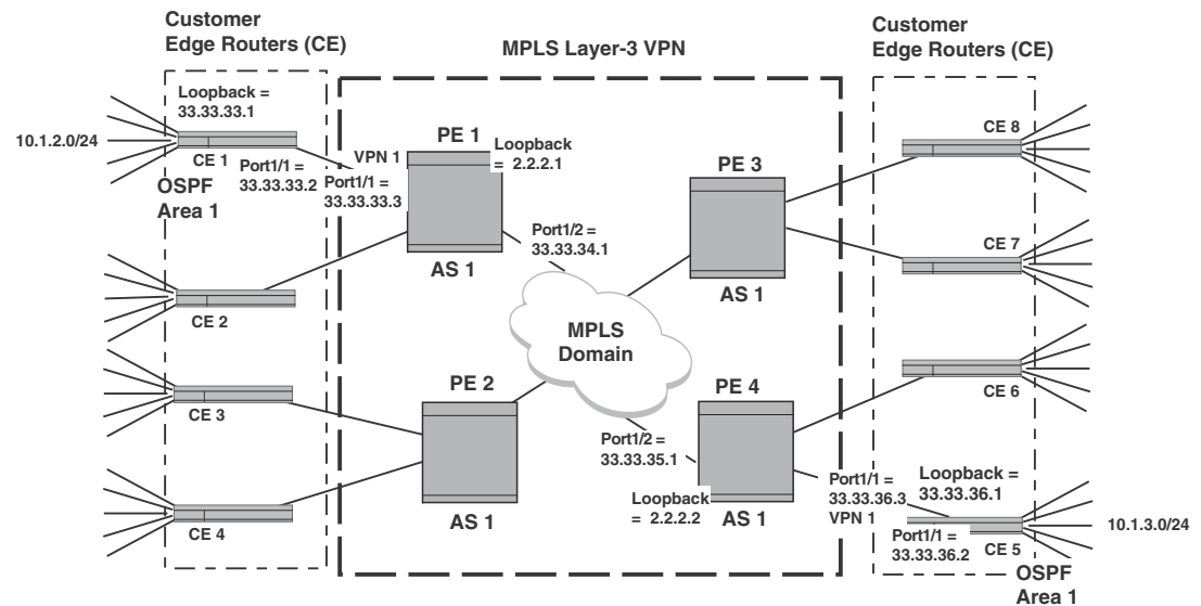
FIGURE 64 Static route to CE network example
