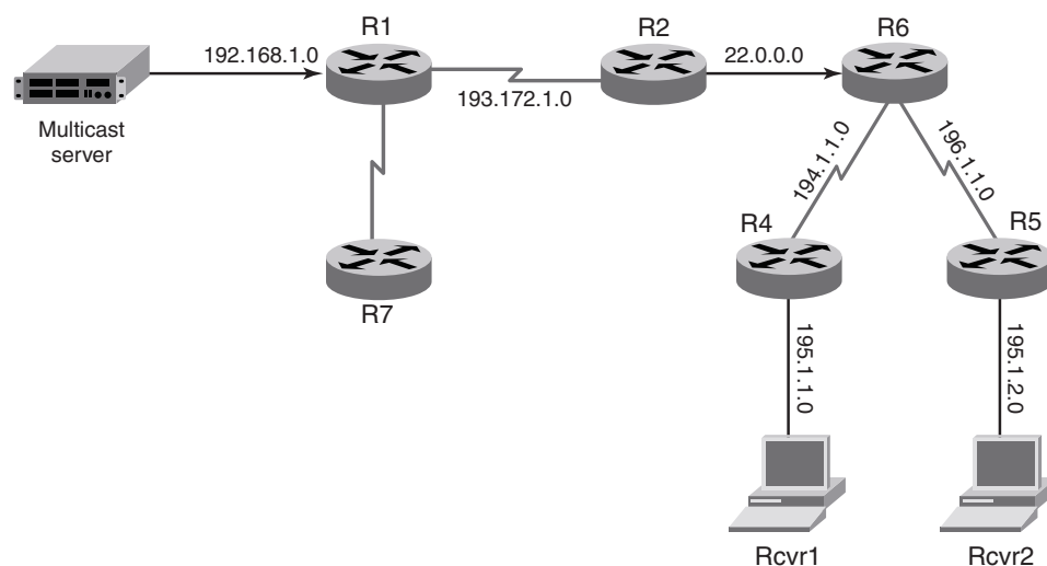
FIGURE 264 Network topology
