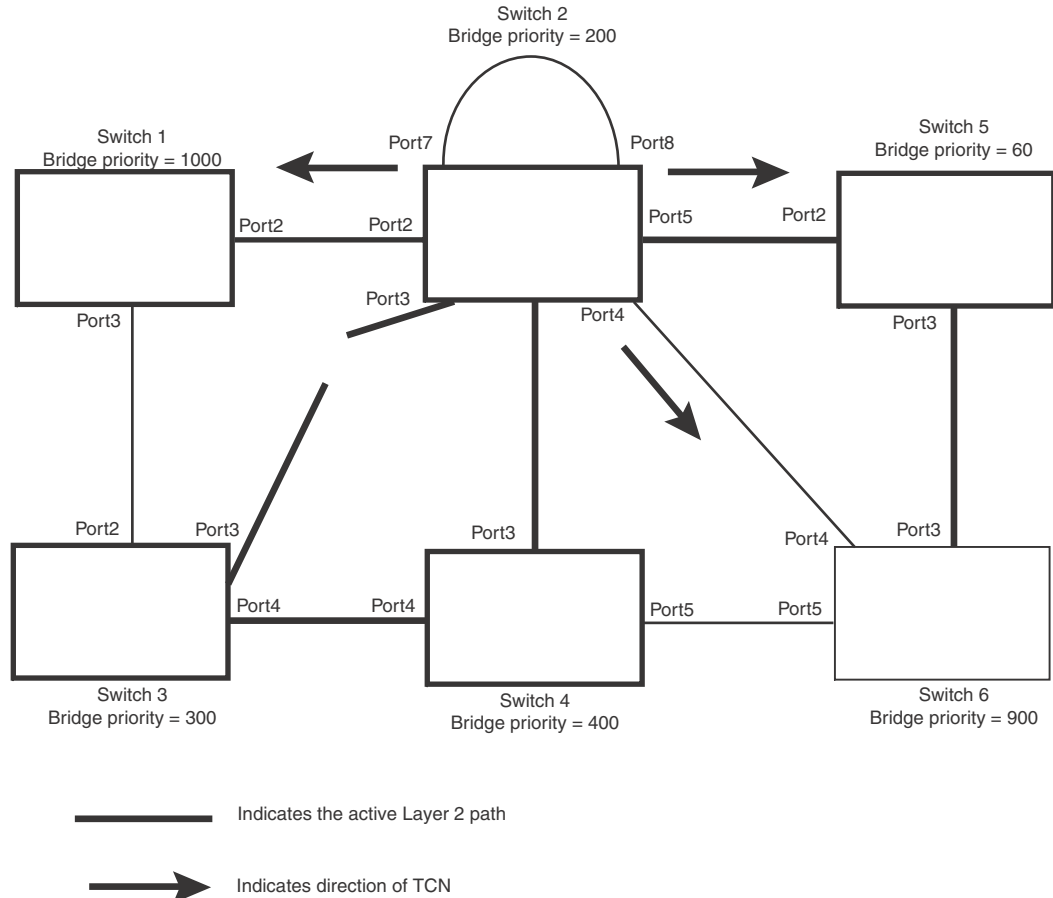
FIGURE 123 Sending TCN to bridges connected to Switch 2
