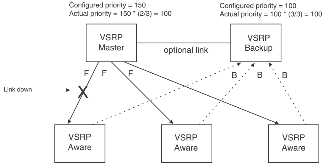
FIGURE 191 VSRP priority bias
