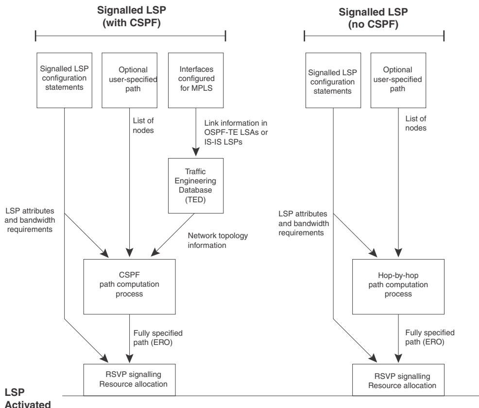
FIGURE 8 How traffic-engineered LSPs are configured, established, and activated
