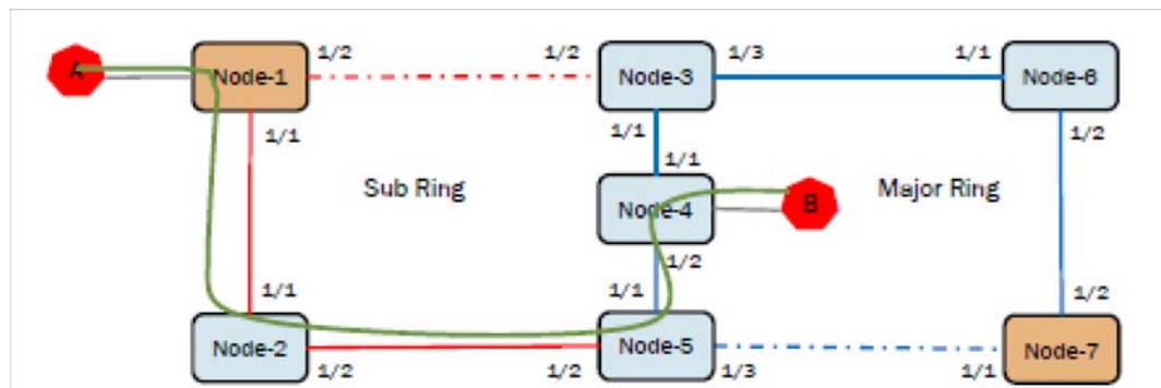
FIGURE 187 RAPS-propagate-tc topology change
