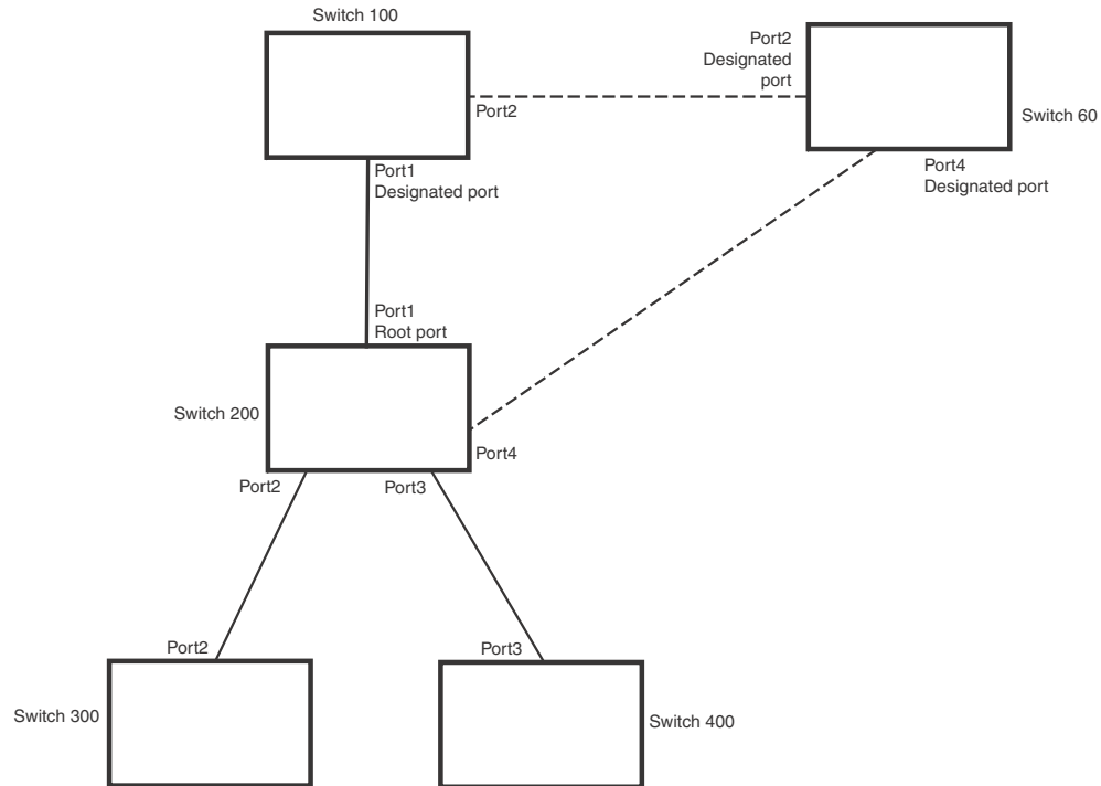
FIGURE 110 Addition of a new root bridge
