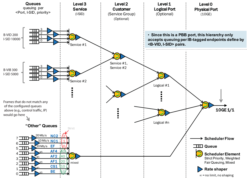
FIGURE 71 PBB HQoS example
