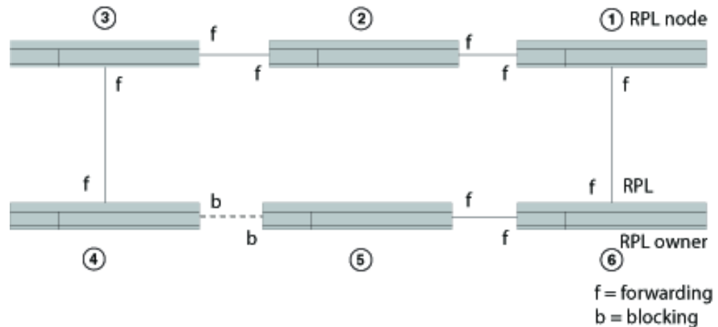
FIGURE 167 ERP topology in a Protected state
