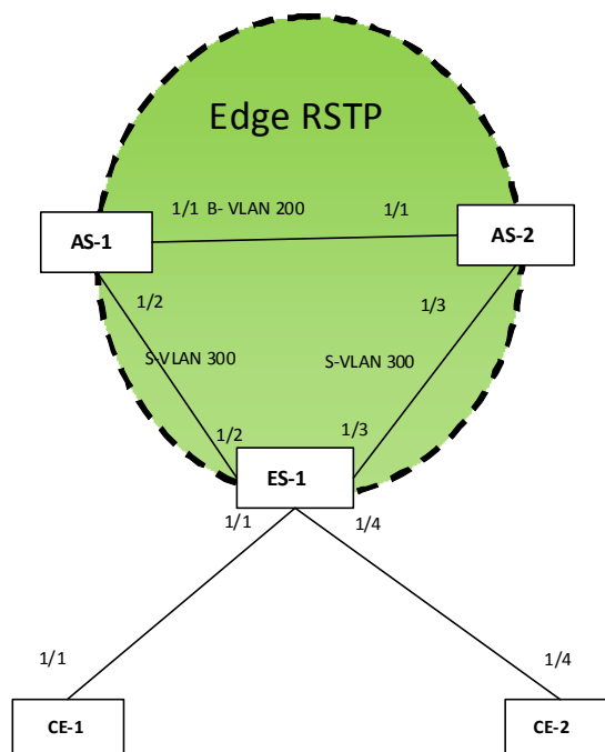
FIGURE 131 Edge RSTP topology 3
