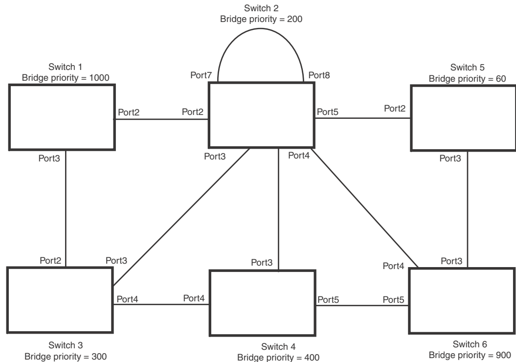
FIGURE 120 Complex RSTP topology
