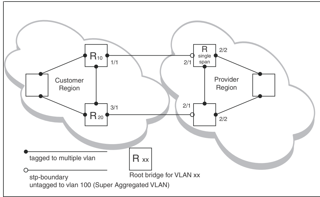
FIGURE 91 Customer using multiple spanning trees and SP using Single STP
