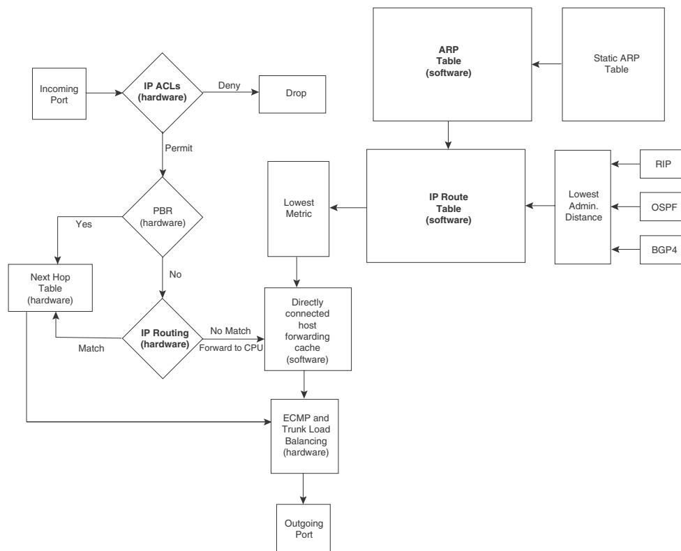
FIGURE 220 IP Packet flow through a Brocade device
