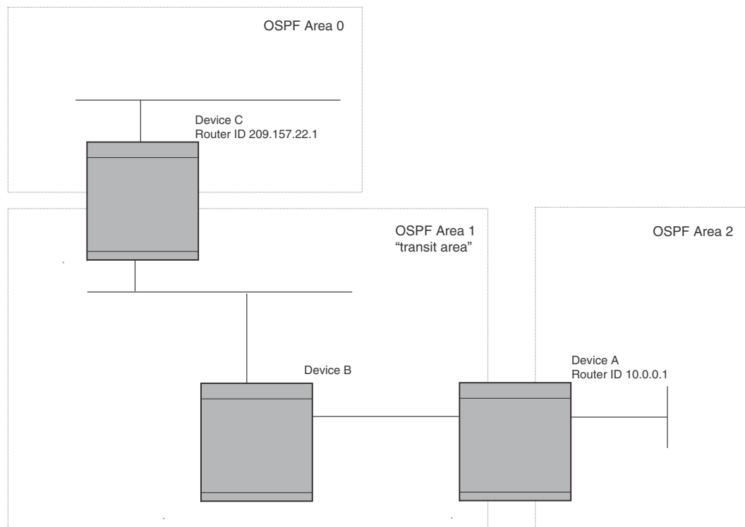
FIGURE 248 Defining OSPF virtual links within a network
