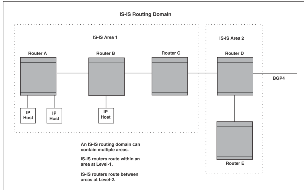
FIGURE 252 An IS-IS network contains Intermediate Systems (ISs) and host systems
