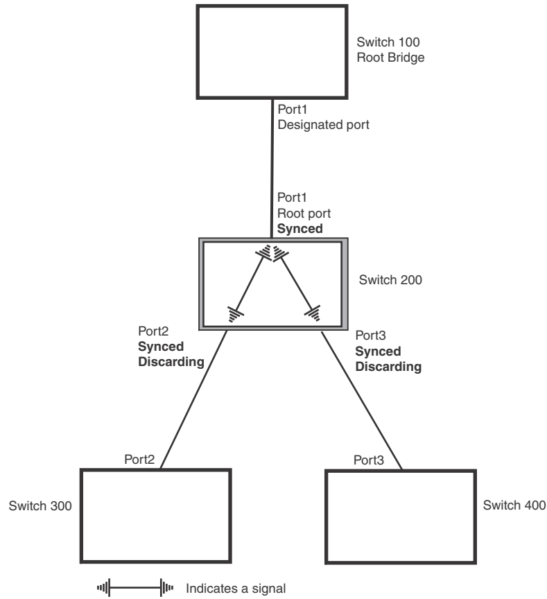
FIGURE 108 Synced stage
