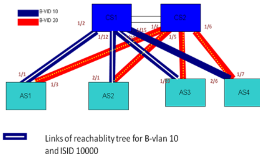
FIGURE 94 Reachability tree for B-VLAN 10 and ISID 10000
