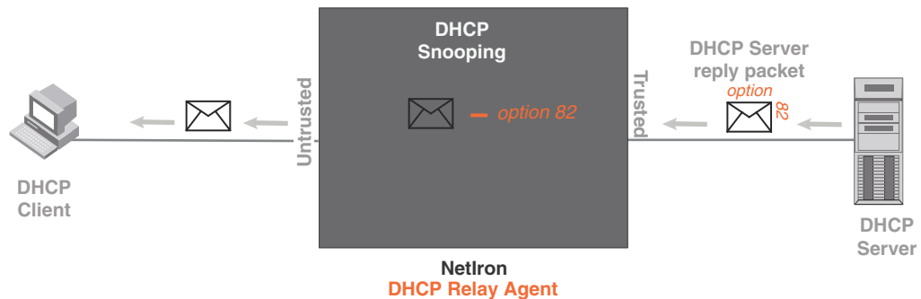
FIGURE 230 DHCP option 82 is removed from the packet
