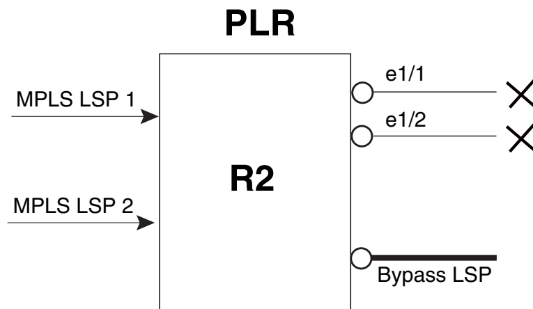
FIGURE 15 Excluded interfaces on a PLR
