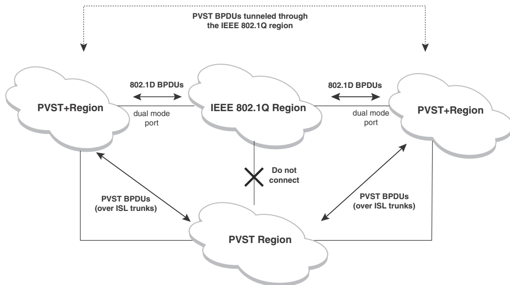
FIGURE 94 Interaction of IEEE 802.1Q, PVST, and PVST+ regions
