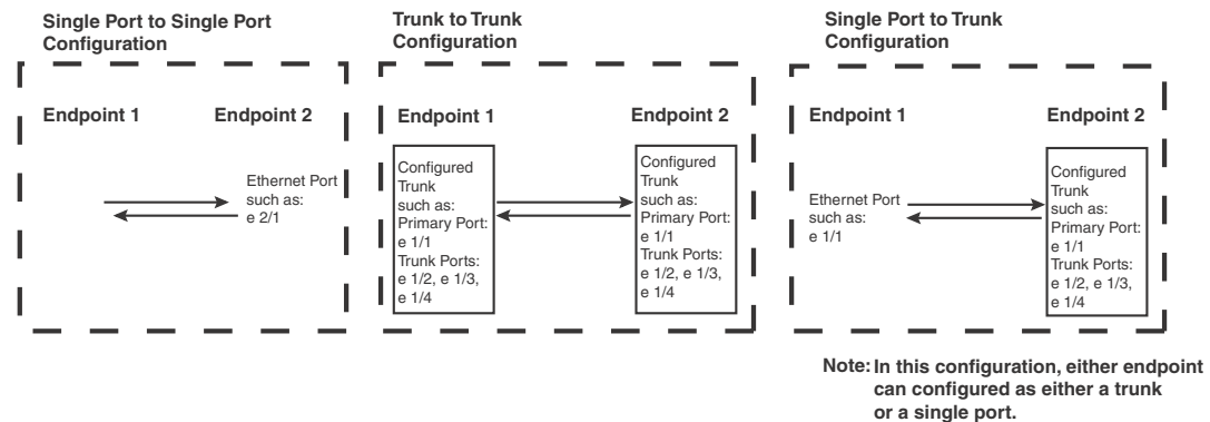
FIGURE 48 Local VLL port and LAG configurations
