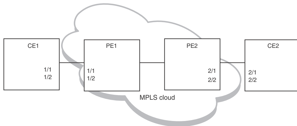
FIGURE 111 - IEEE 802.1ag over VLL scenerio
