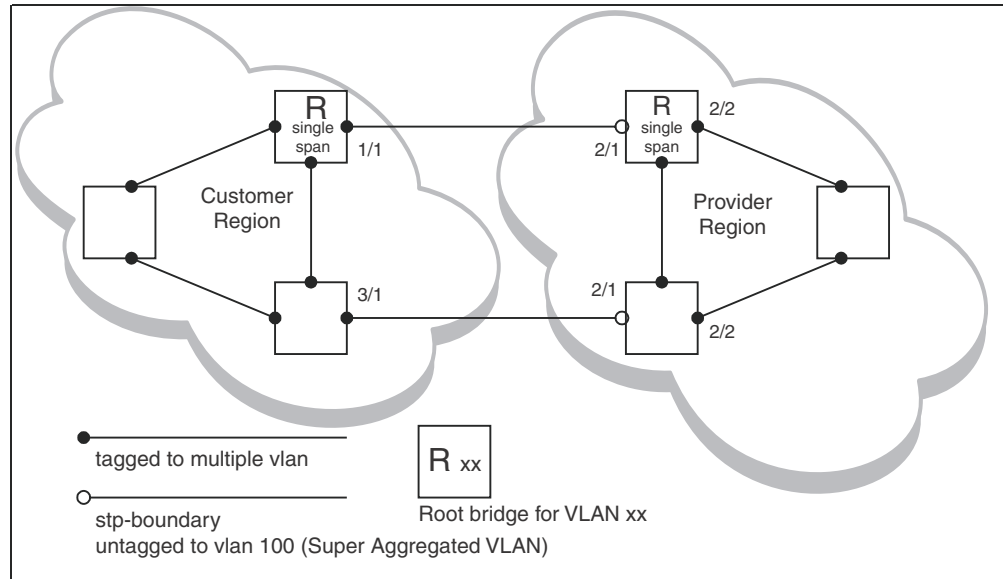
FIGURE 93 Customer and SP using Single STP
