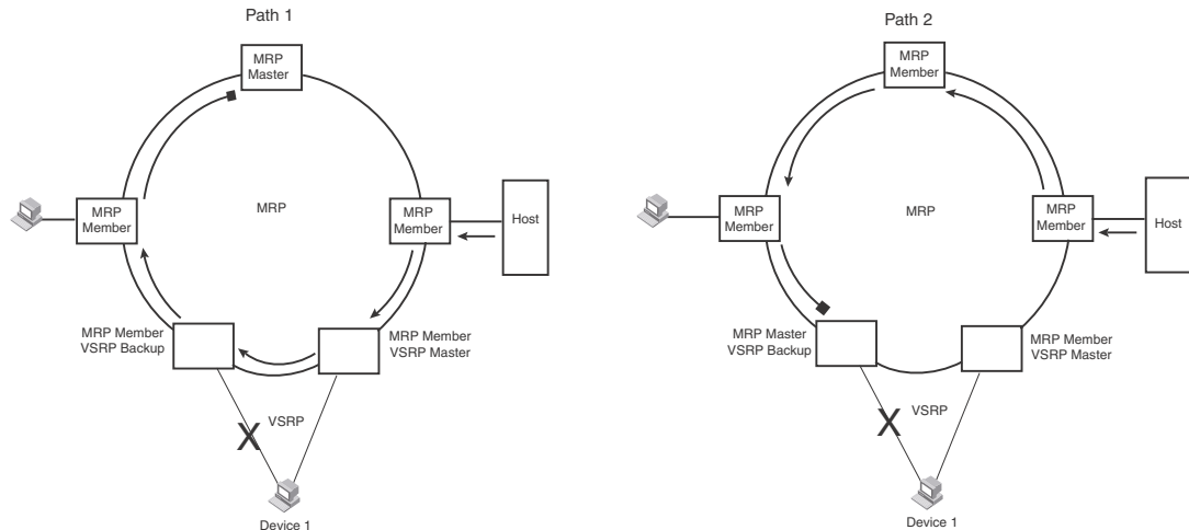
FIGURE 199 VSRP on Foundry MRP rings that failed over
