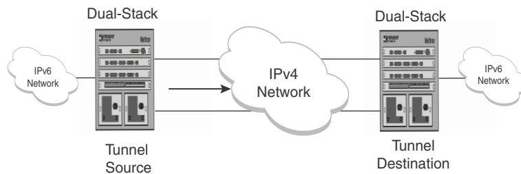
FIGURE 237 Manually configured tunnel
