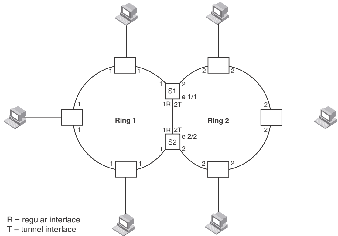
FIGURE 149 Interface IDs and types
