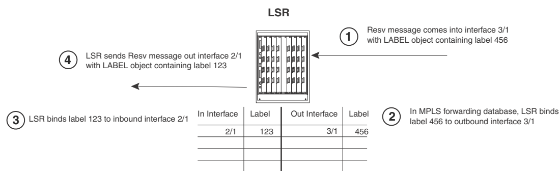
FIGURE 10 How the RSVP LABEL object associates a label with an interface in the MPLS forwarding table
