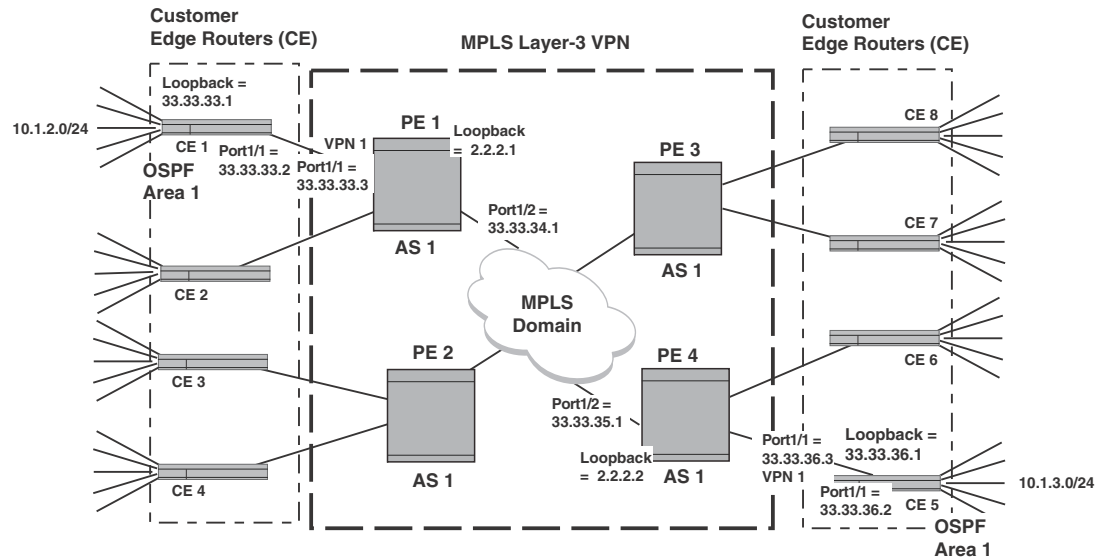
FIGURE 65 RIP to CE network example
