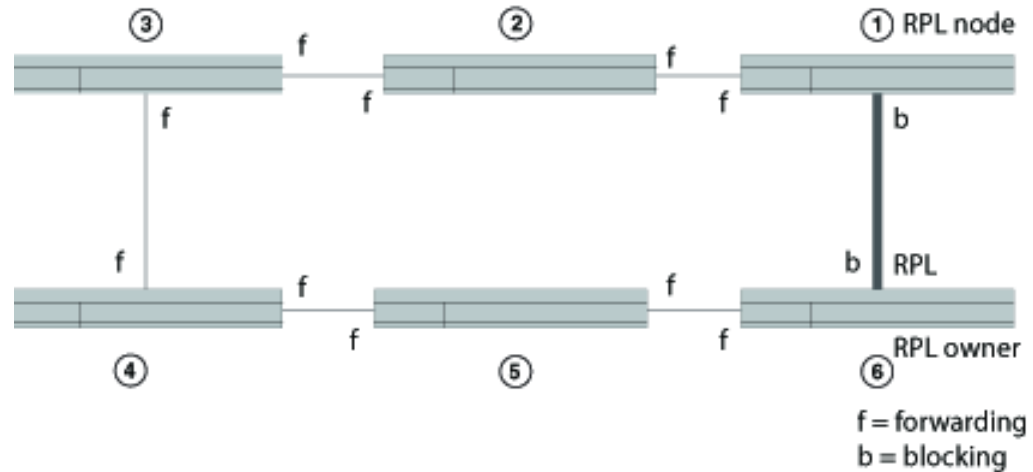
FIGURE 166 ERP topology
