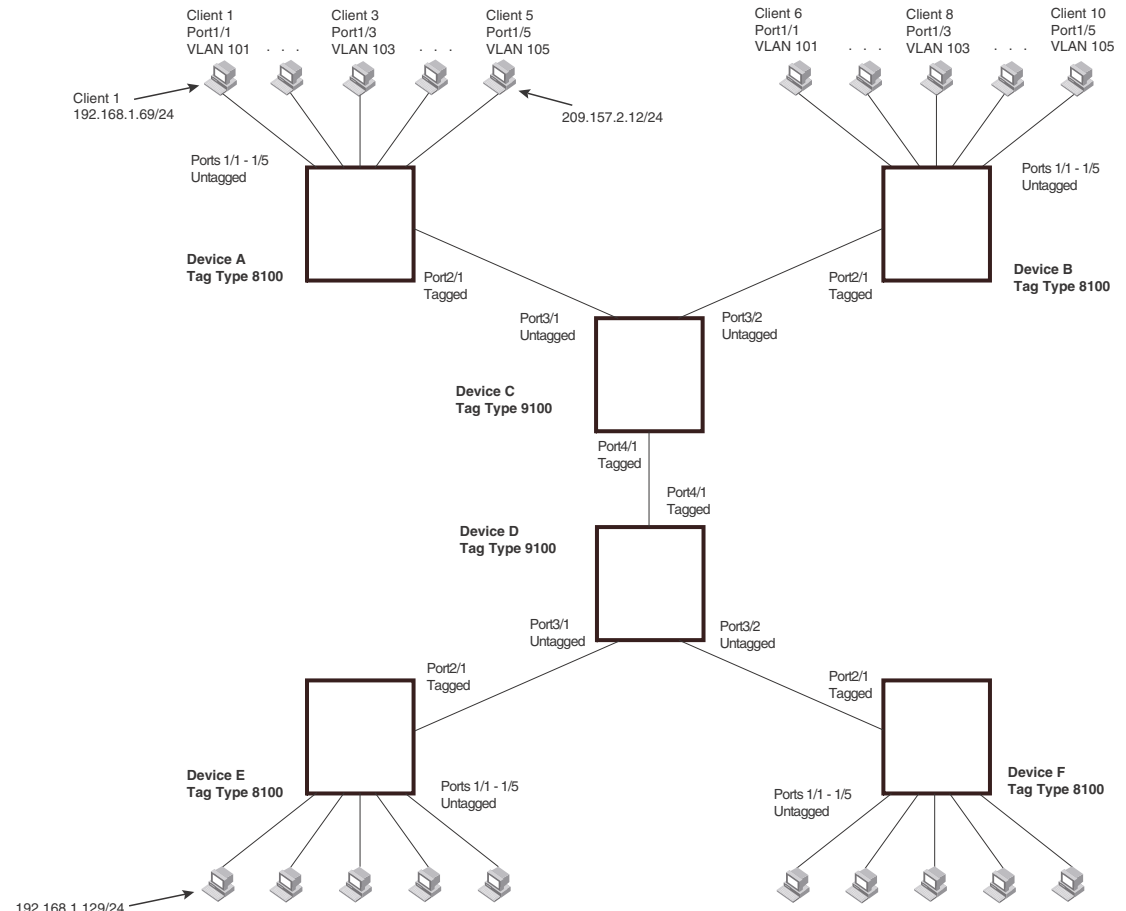
FIGURE 14 Example super aggregated VLAN application
