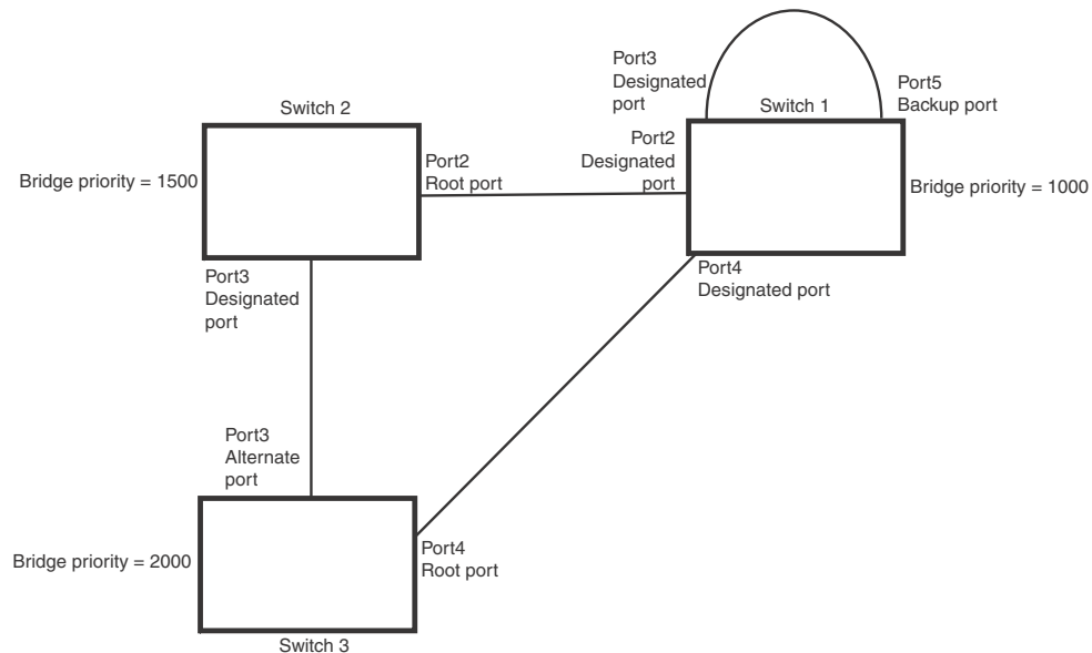
FIGURE 117 Simple Layer 2 topology
