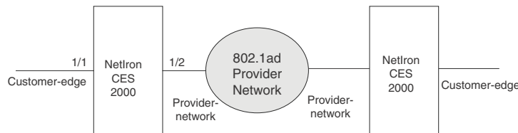
FIGURE 25 Port types in a Provider Bridge (PB)
