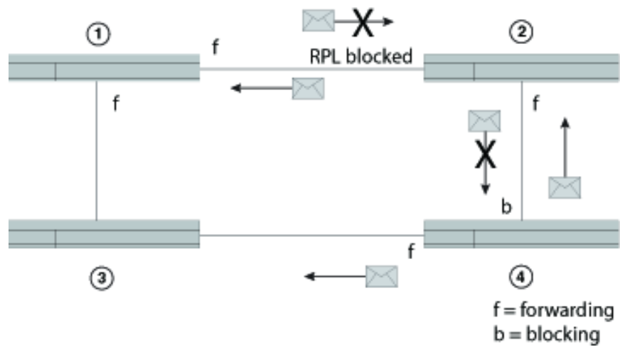
FIGURE 164 Initializing an ERP topology - VI
