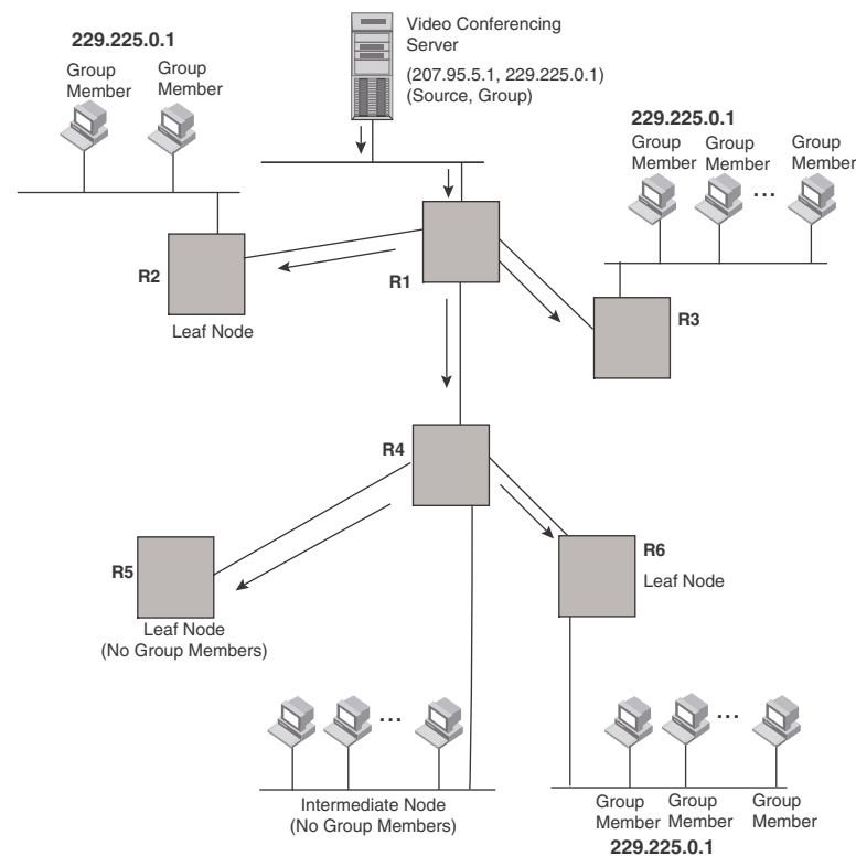
FIGURE 266 Pruning leaf nodes from a multicast tree
