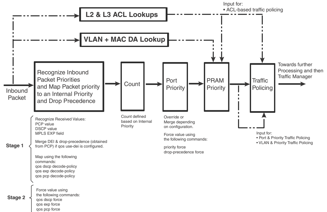
FIGURE 59 Logic flow of Ingress QoS processing
