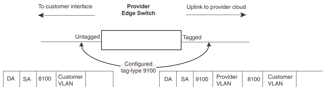
FIGURE 15 SAV configuration example
