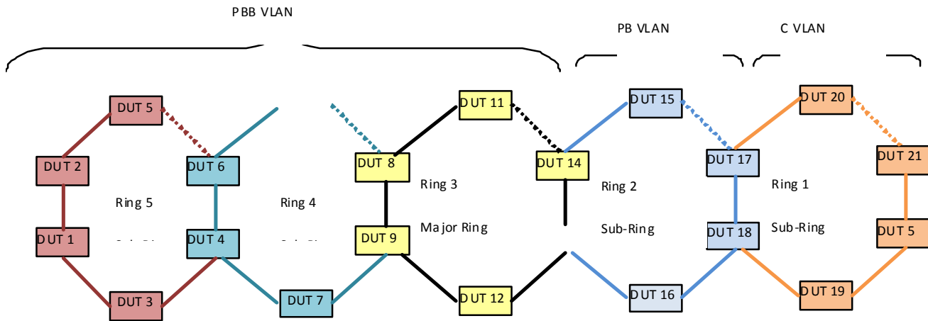
FIGURE 176 ERP configuration over ESI network
