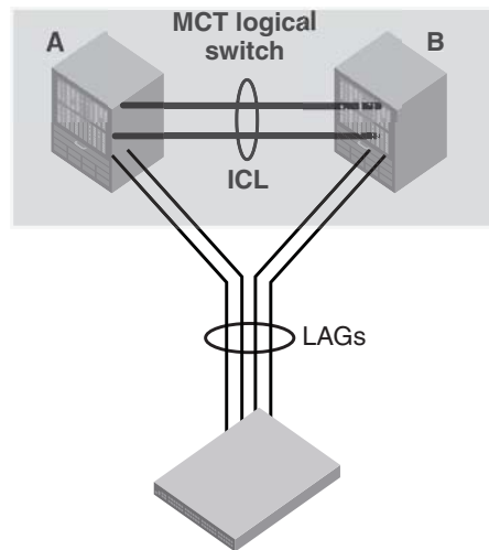
FIGURE 208 MCT peers
