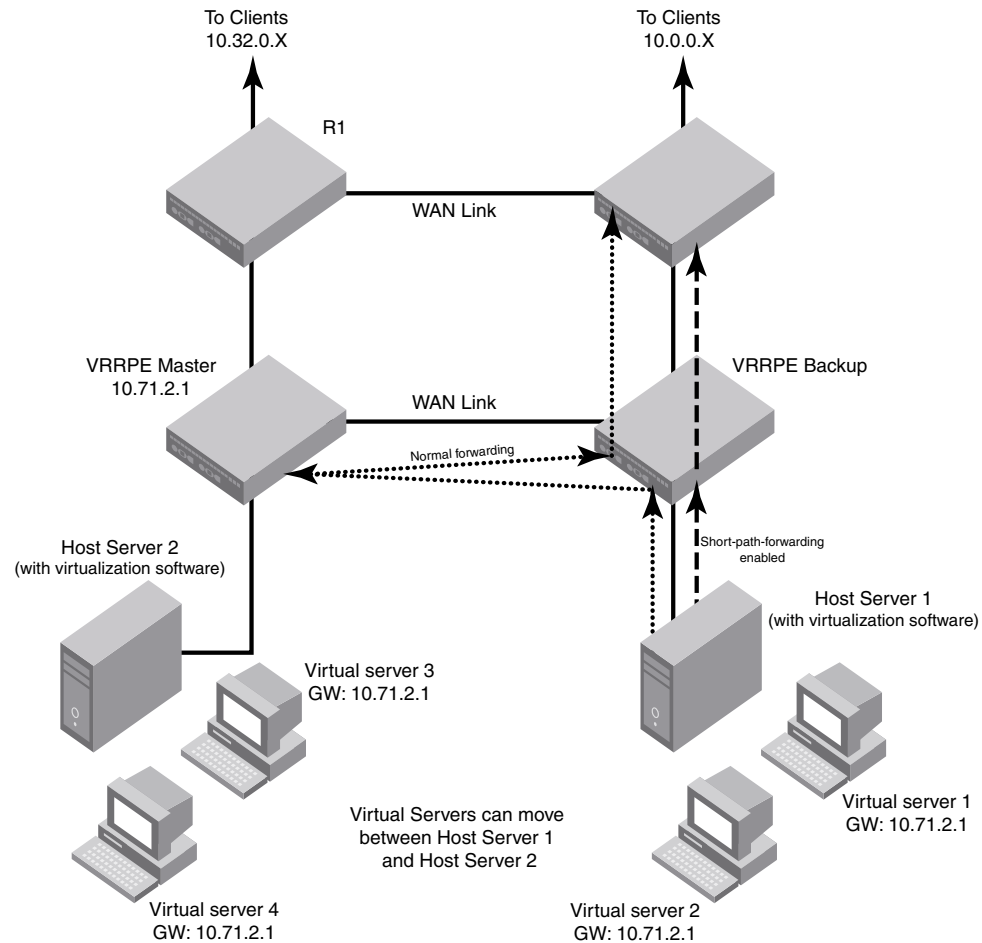
FIGURE 204 Short path forwarding
