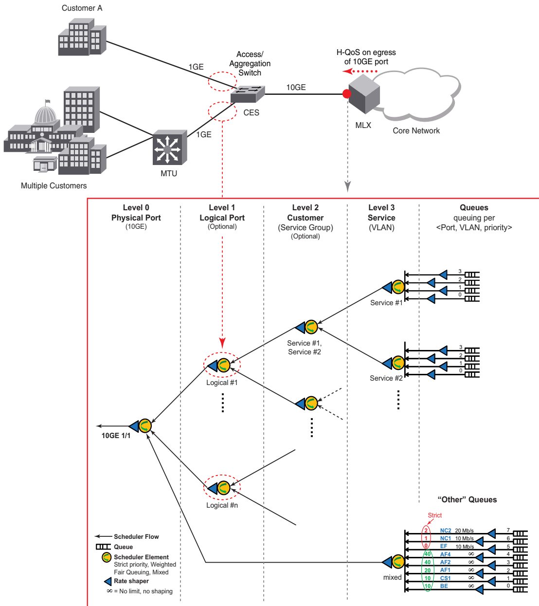
FIGURE 68 HQoS towards the Customers
