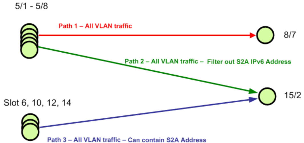
FIGURE 242 Configuration example 3
