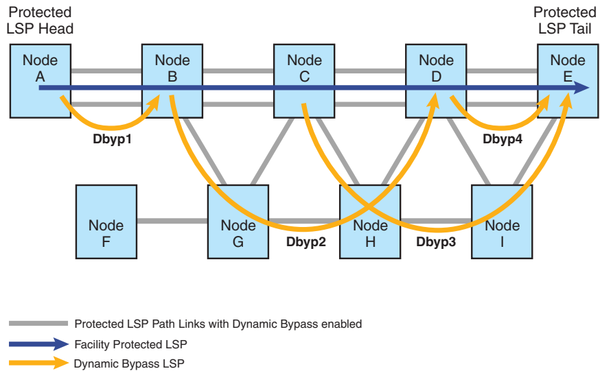
FIGURE 30 Dynamic bypass creation with link protection PLRs.a
