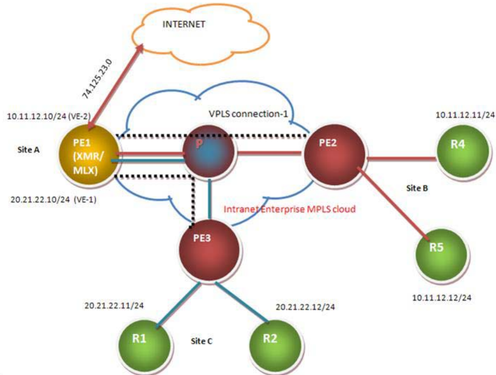
FIGURE 75 Routing over VPLS topology
