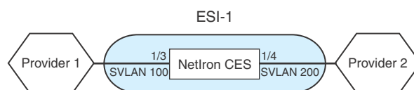
FIGURE 27 SVLAN translation at an inter-provider boundary
