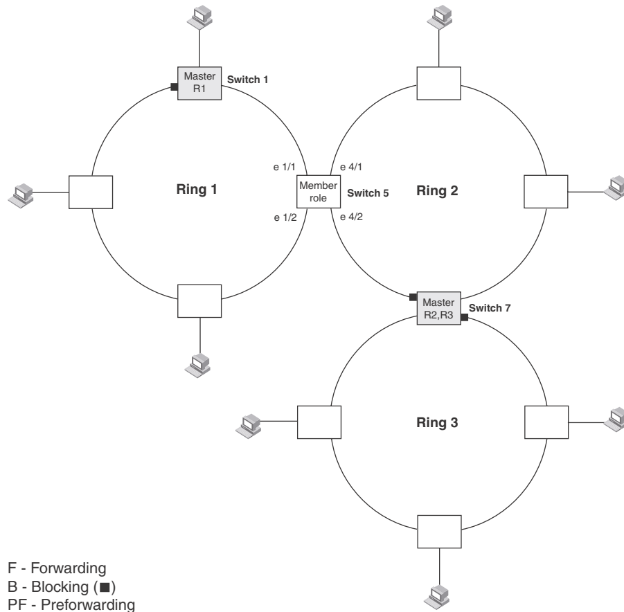
FIGURE 145 Multiple MRP rings - phase 1
