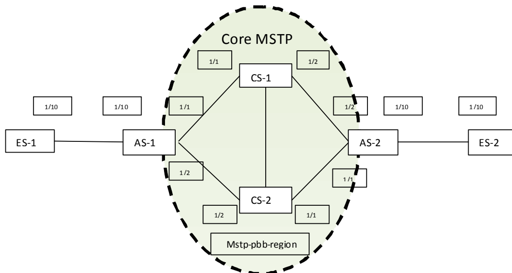
FIGURE 102 Core MSTP in a PBB network
