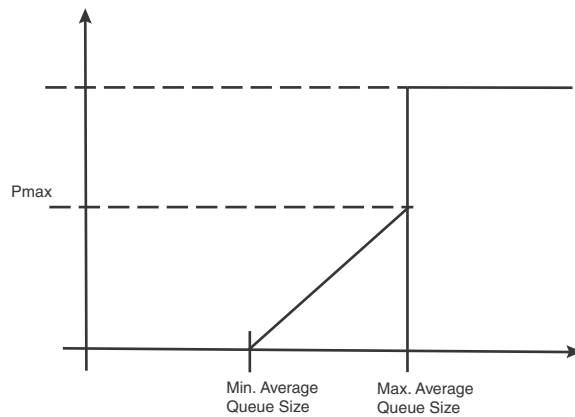
FIGURE 63 WRED operation graph
