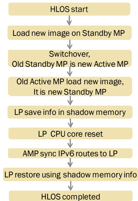
FIGURE 83 IPv6 HLOS operation
