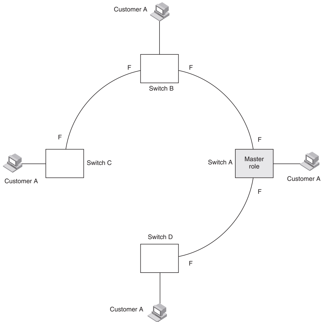
FIGURE 140 MRP ring – ring break
