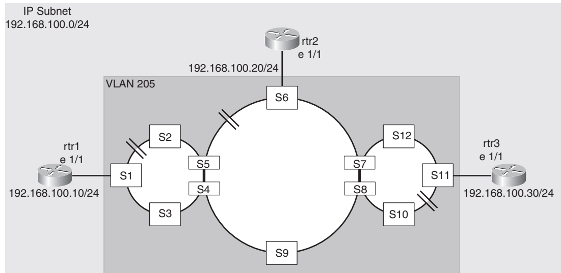
FIGURE 147 Multiple rings with one vlan spanning them
