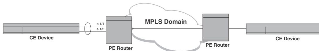
FIGURE 46 Specifying a LAG group as the endpoint of a VLL
