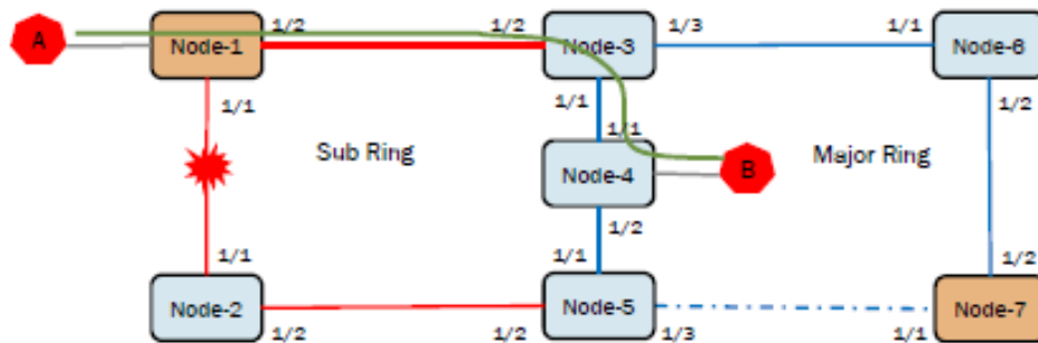
FIGURE 187 RAPS-propagate-tc topology change
