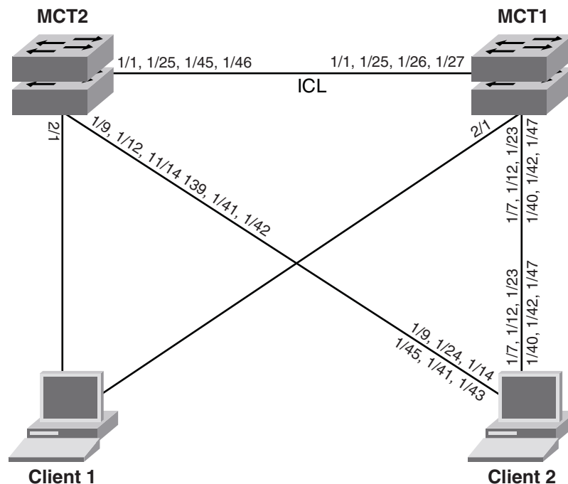
FIGURE 218 MCT snooping topology example
