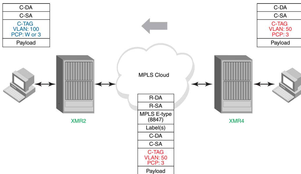
FIGURE 54 Sample configuration
