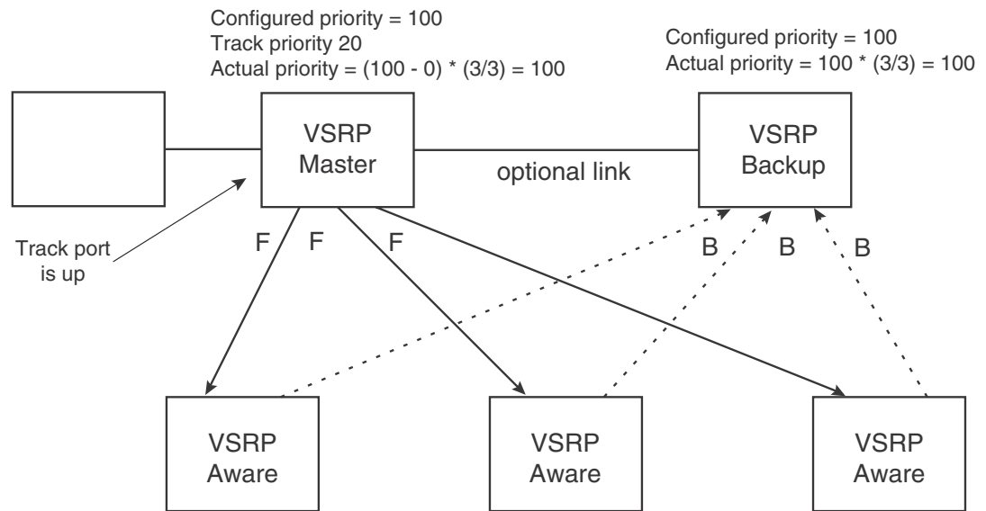
FIGURE 192 Track port priority
