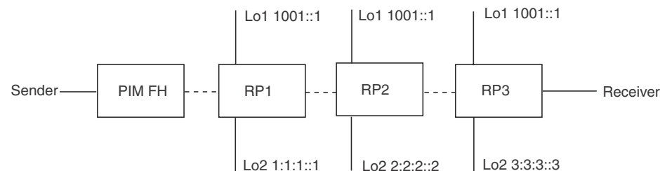
FIGURE 90 Example of a PIM Anycast RP network
