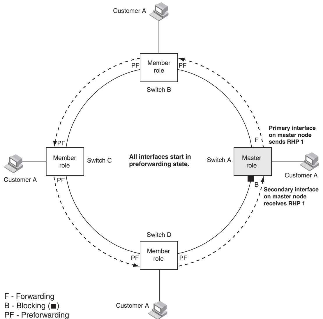
FIGURE 138 MRP ring – initial state
