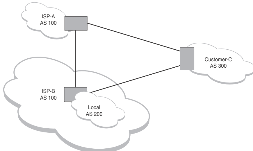
FIGURE 260 Example of Local AS configured on ISP-B
