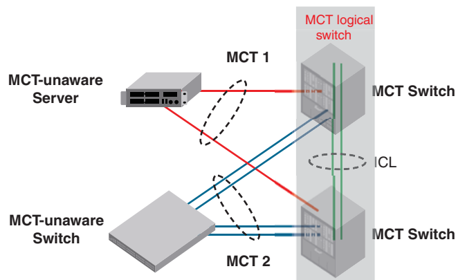
FIGURE 205 Chassis trunk example
