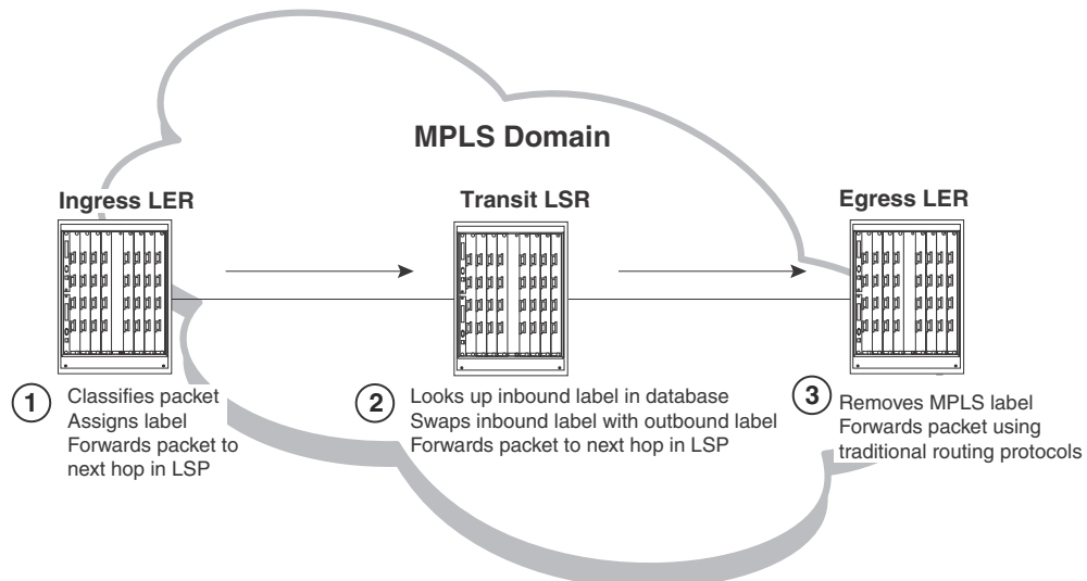
FIGURE 4 Label switching in an MPLS domain
