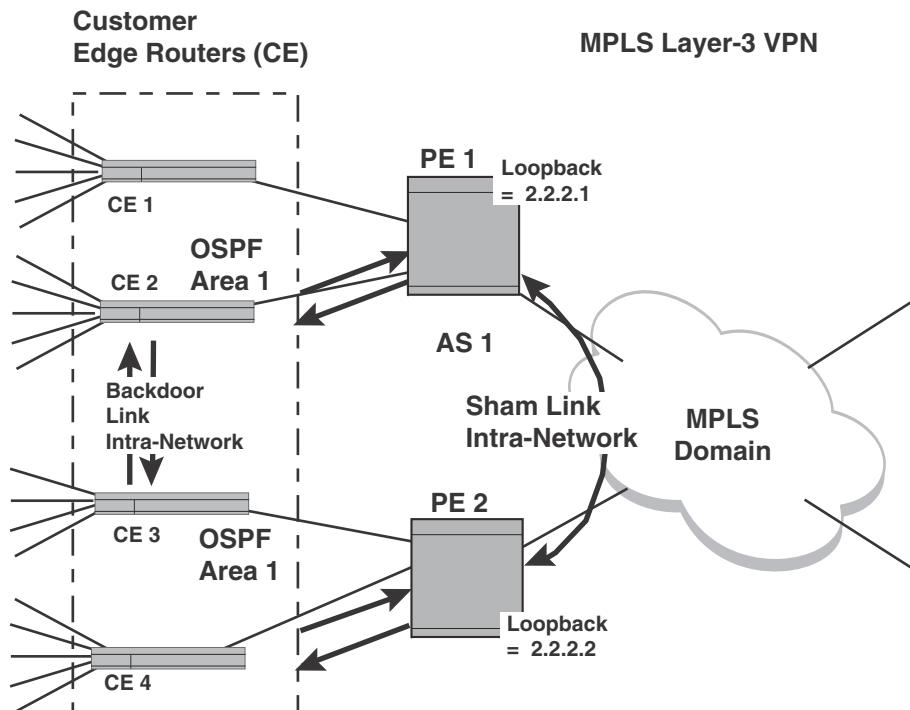
FIGURE 72 BGP or MPLS VPN with OSPF including Sham link and backdoor link
