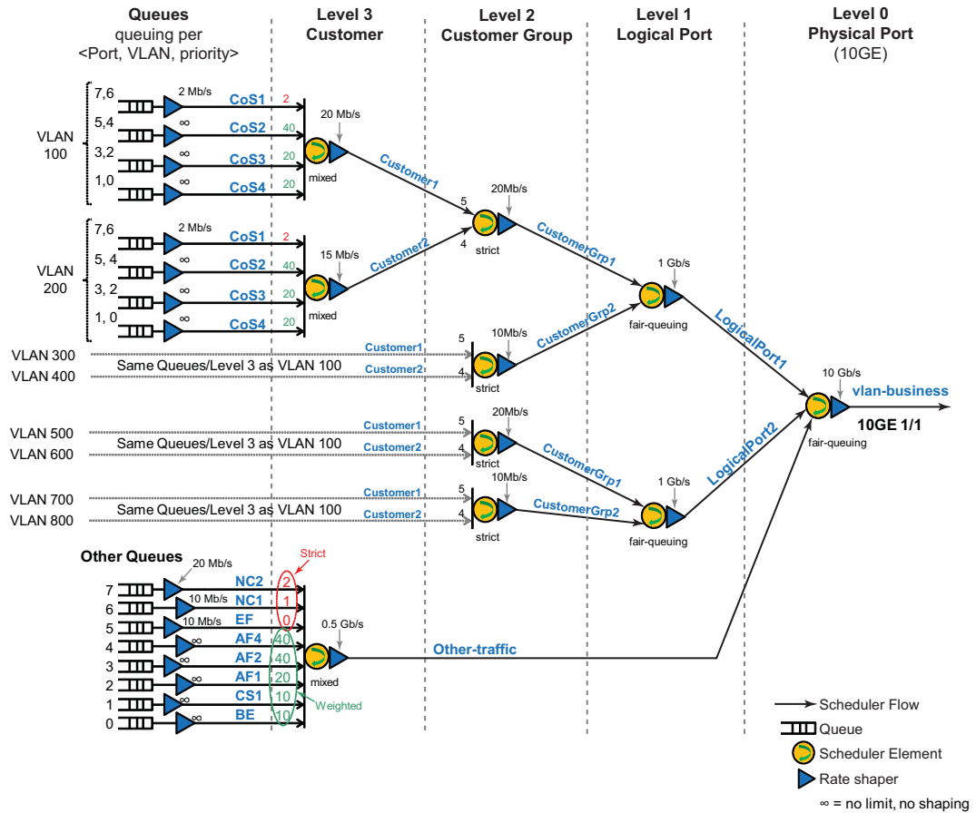
FIGURE 79 VLAN HQoS deployment example
