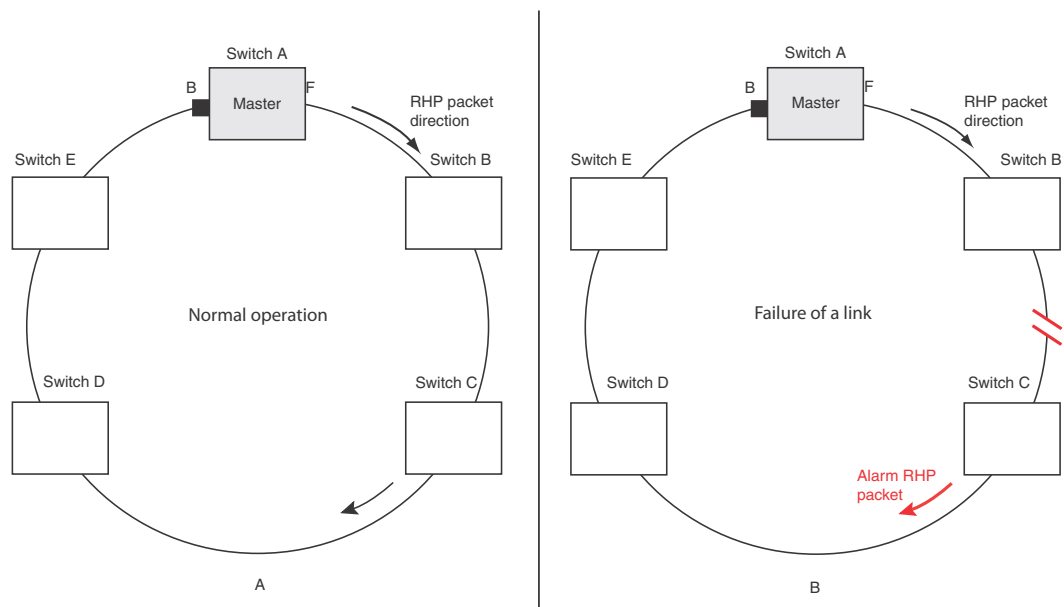
FIGURE 141 An MRP ring under normal operation (A) and after detection of a failure in the ring (B)
