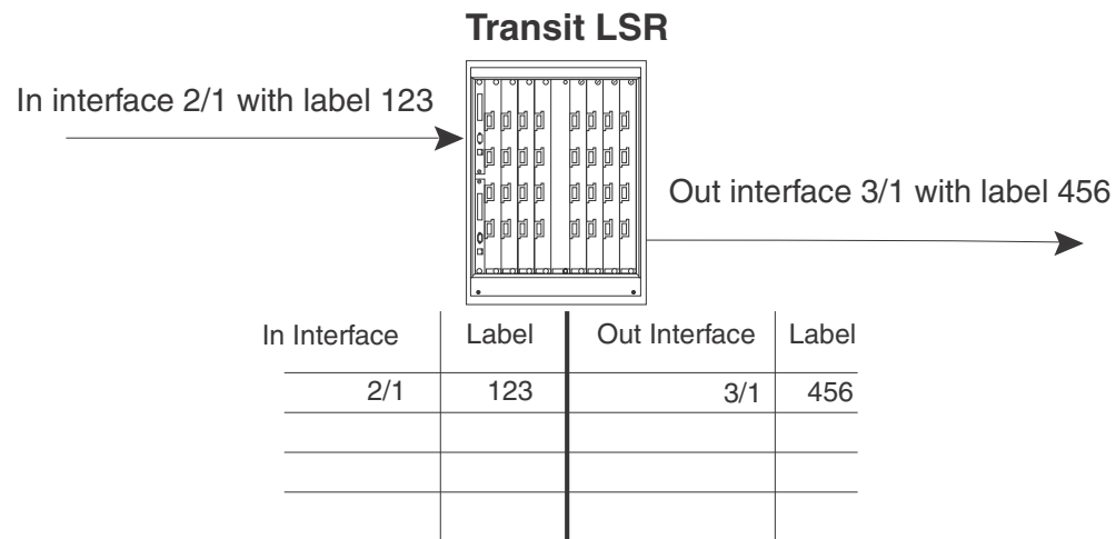
FIGURE 39 Sample LDP configuration
