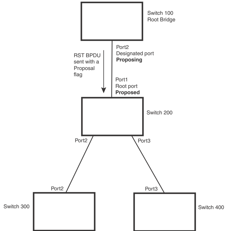
FIGURE 106 Proposing and proposed stage
