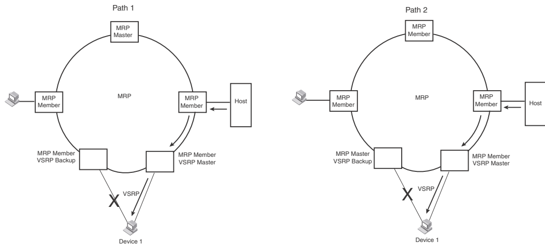
FIGURE 200 New path established
