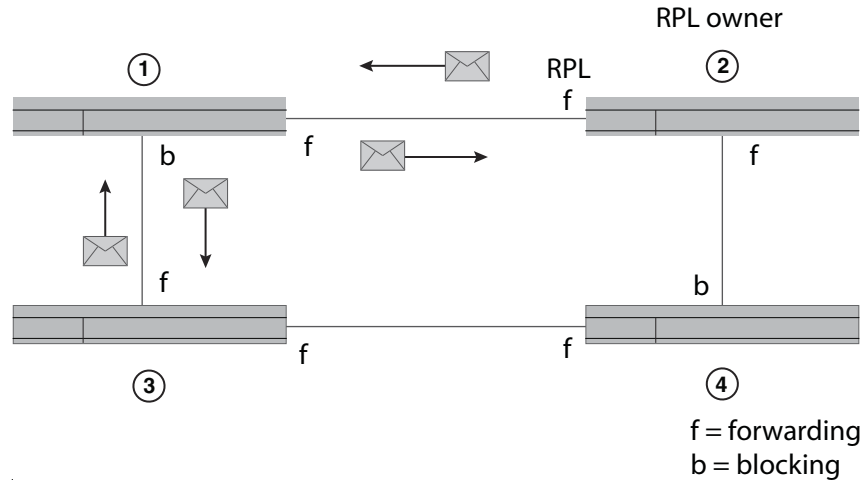
FIGURE 160 Initializing an ERP topology - II
