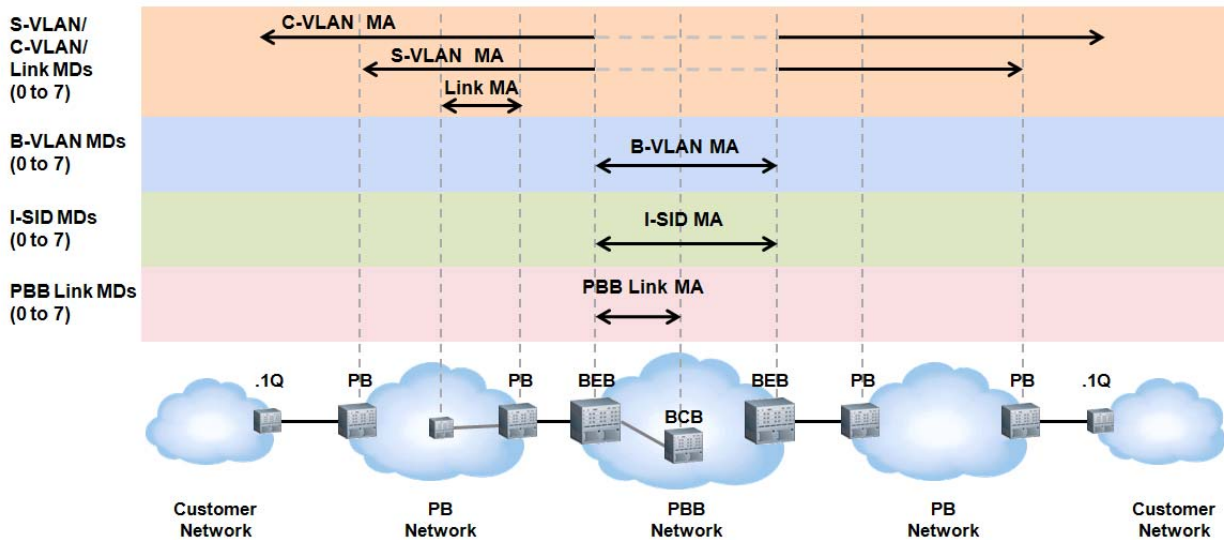
S-VLAN, C-VLAN, and Link MAs (Figure 54)
