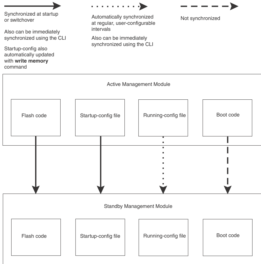
FIGURE 3 Active and standby management module file synchronization
