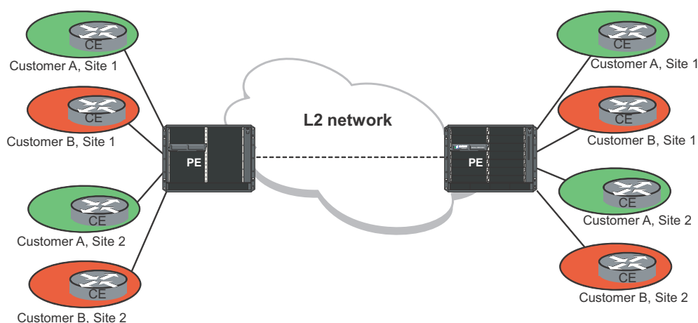
FIGURE 279 A Network deploying Multi-VRF
