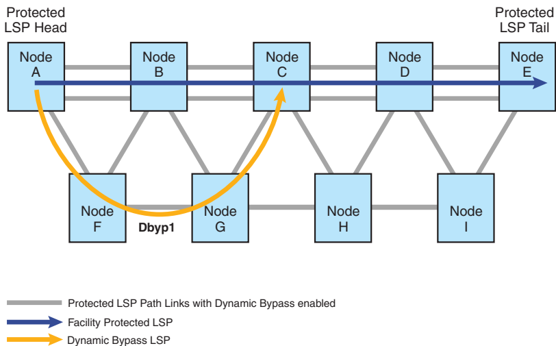
FIGURE 25 Automatic creation of dynamic creation and merge point selection
