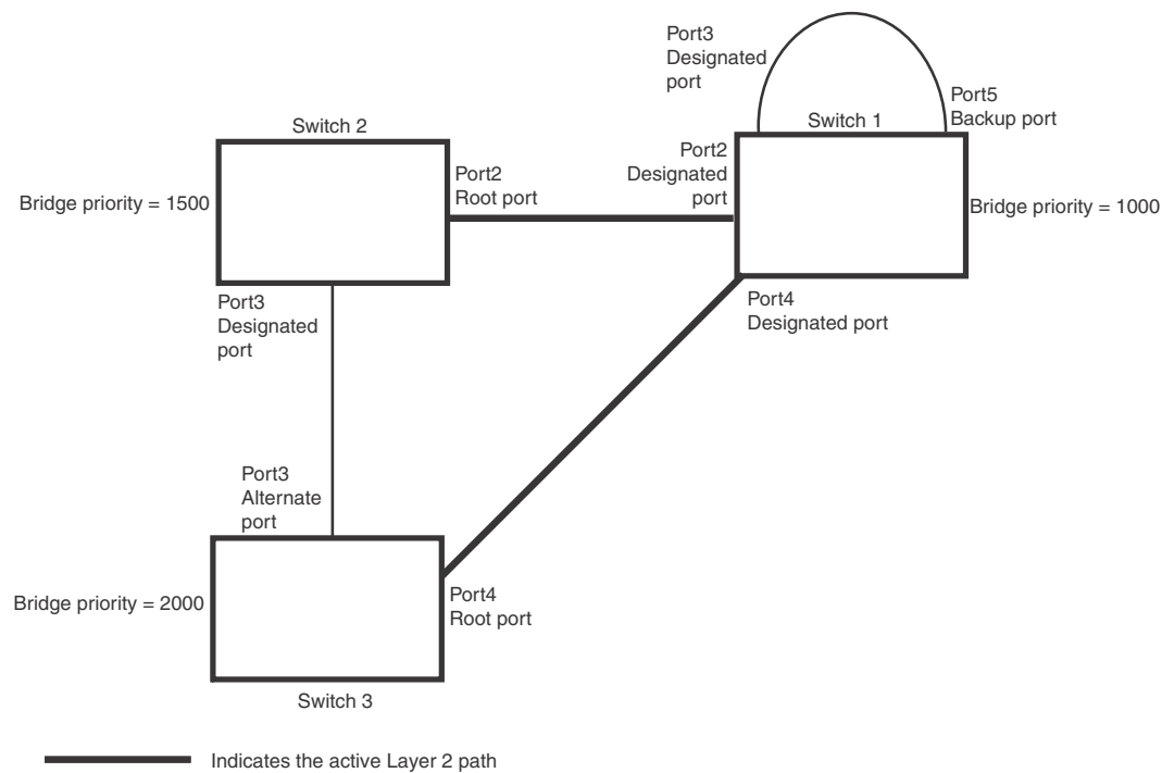
FIGURE 118 Active Layer 2 path
