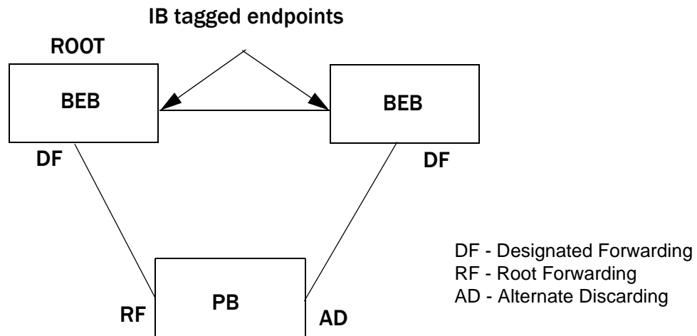
FIGURE 128 RSTP convergence when two AS connected via IB tagged endpoint
