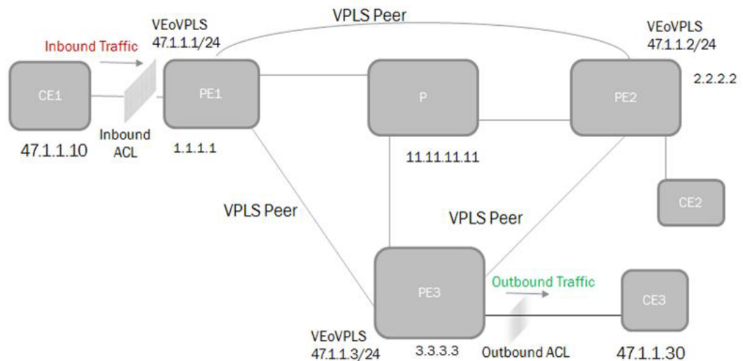
FIGURE 77 Sample VE over VPLS topology using ACLs
