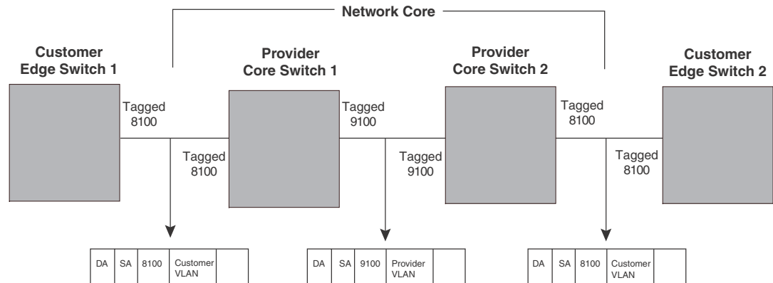
FIGURE 18 802.1q Tag-type translation configuration example 1
