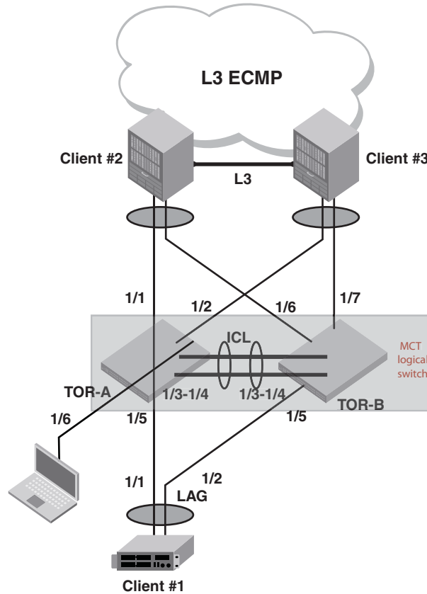
FIGURE 212 Single level MCT- extension
