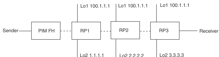
FIGURE 271 Example of a PIM Anycast RP network
