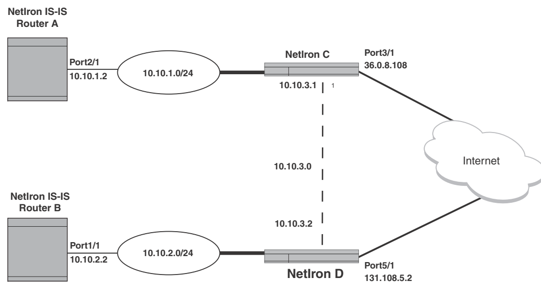
FIGURE 256 IS-IS over a GRE IP tunnel
