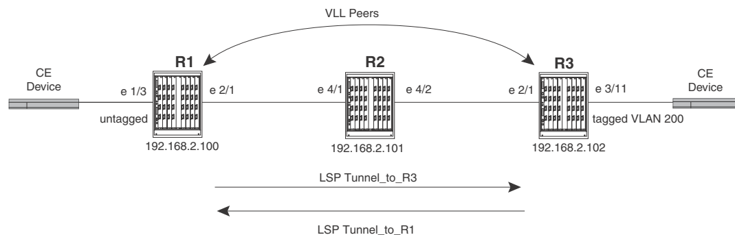
FIGURE 47 MPLS VLL configuration
