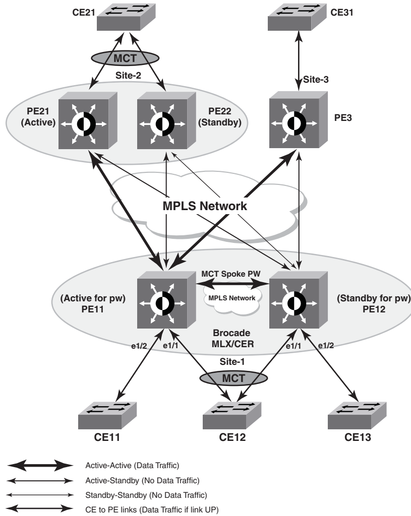
FIGURE 216 Sample topology with MCT end-points for VPLS
