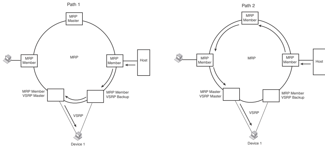
FIGURE 198 Two data paths from host on a Foundry MRP ring to a VSRP-linked device
