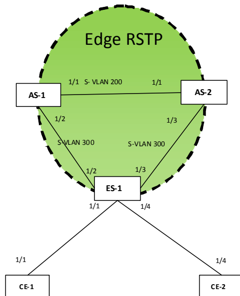
FIGURE 133 Edge RSTP topology 5
