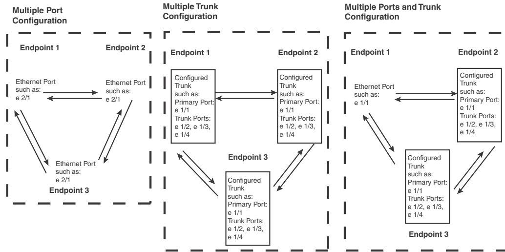
FIGURE 55 Local VPLS port and LAG configurations
