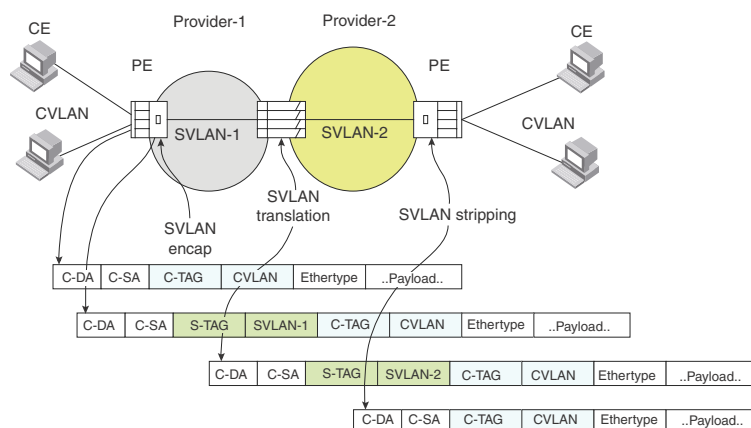
FIGURE 24 IEEE 802.1ad network
