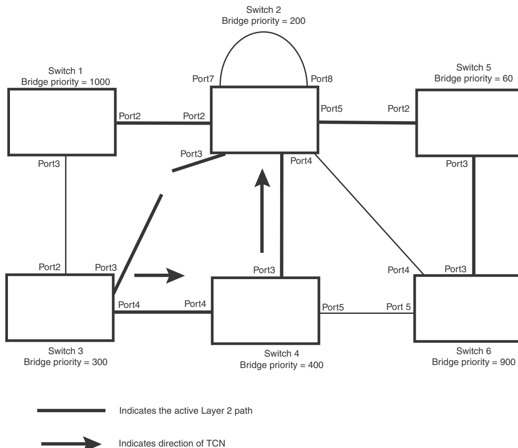
FIGURE 122 Beginning of topology change notice
