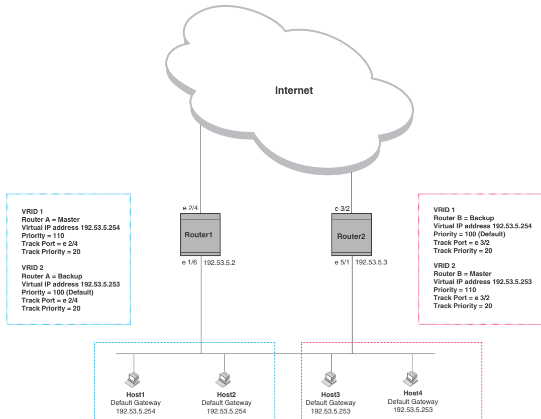
FIGURE 203 Router1 and Router2 are configured to provide dual redundant network access for the host
