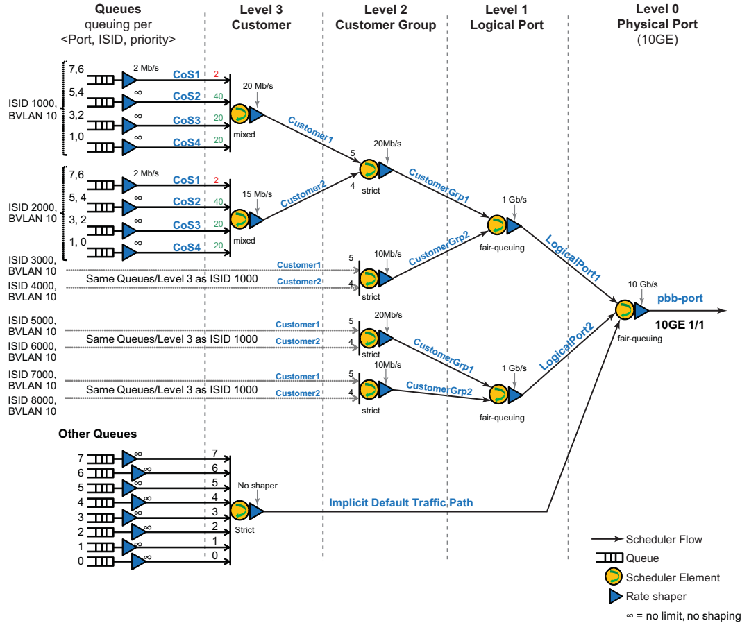
FIGURE 78 PBB HQoS mode
