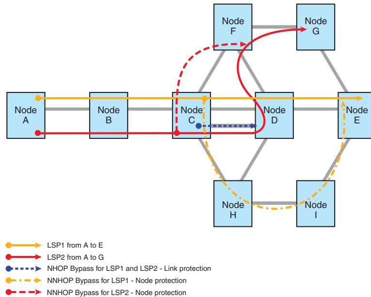
FIGURE 22 Two facility protected LSPs using a common link
