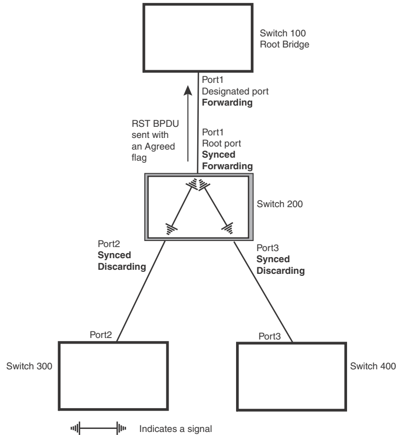
FIGURE 109 Agree stage
