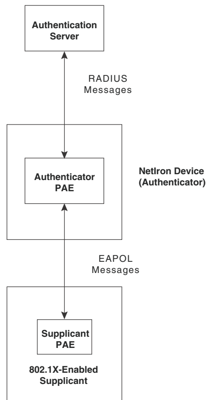
FIGURE 97 Authenticator PAE and supplicant PAE
