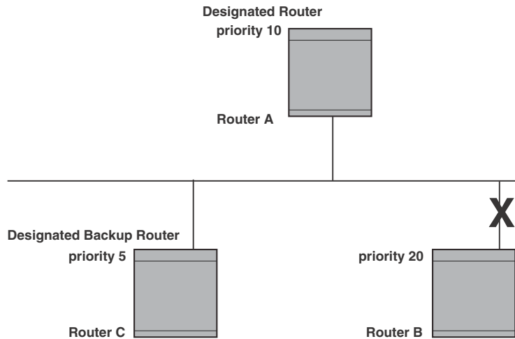
FIGURE 245 Backup designated router becomes designated router
