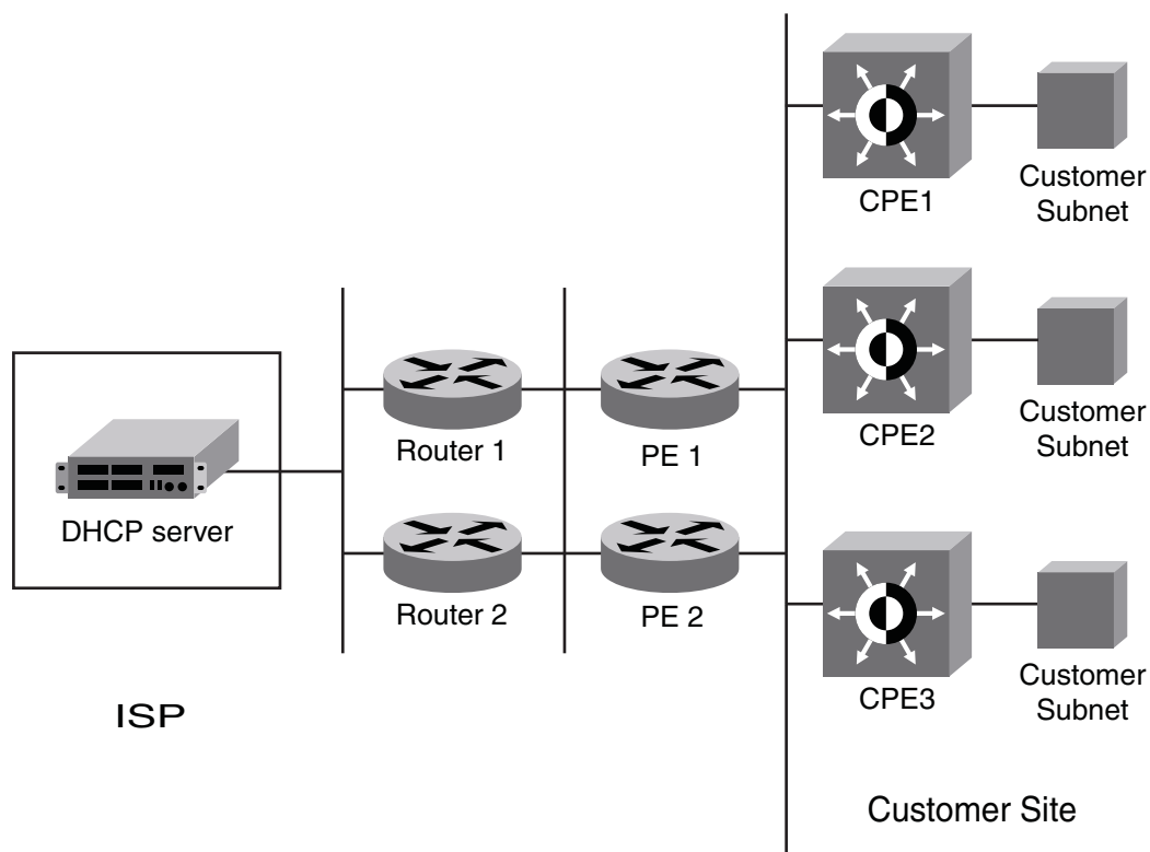
FIGURE 84 DHCPv6 Relay Agent Prefix Delegation Notification
