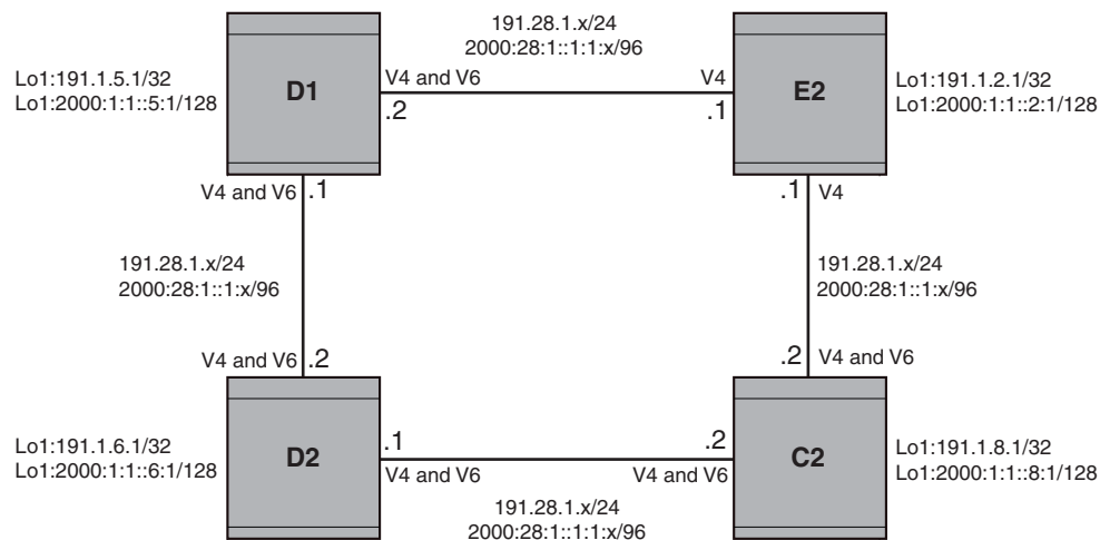
FIGURE 88 IPv6 IS-IS MT configuration
