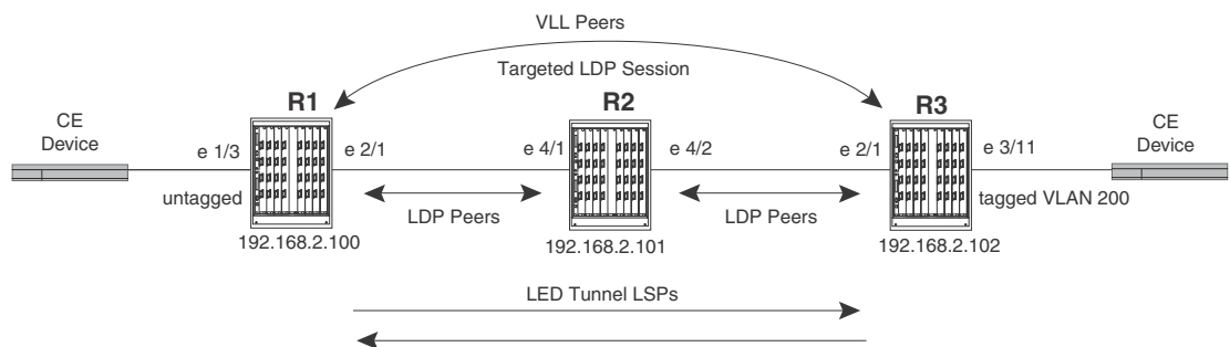
FIGURE 40 MPLS VLL configuration with LDP tunnel LSPs
