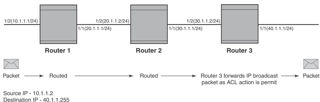
FIGURE 239 Filtering of IP directed broadcast traffic on the Router 3 interface
