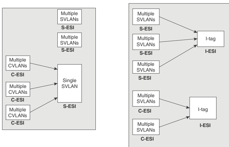
PB 802.1ad: SVLANs bound to different provider S-ESIs need to be unique, whether or not connected with C-ESIs
