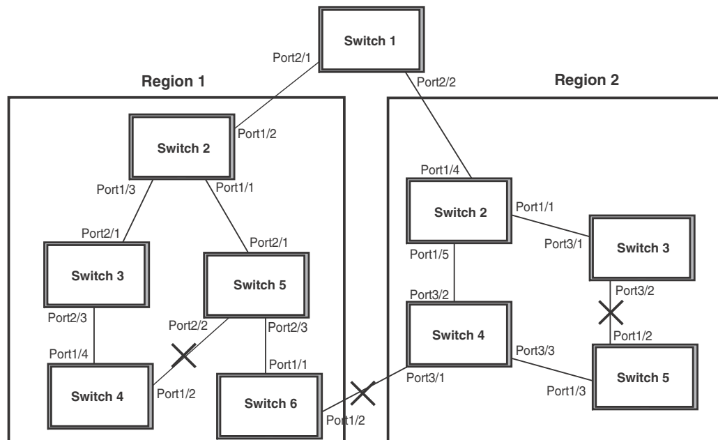
FIGURE 97 MSTP configured network
