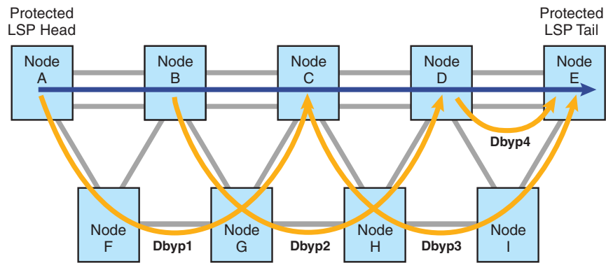
FIGURE 29 Dynamic bypass creation from all PLRs
