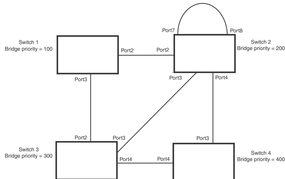
FIGURE 103 Simple RSTP topology
