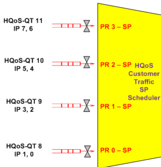
FIGURE 84 SP scheduling model for HQoS other traffic
