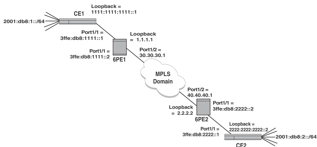
FIGURE 81 Deploying 6PE
