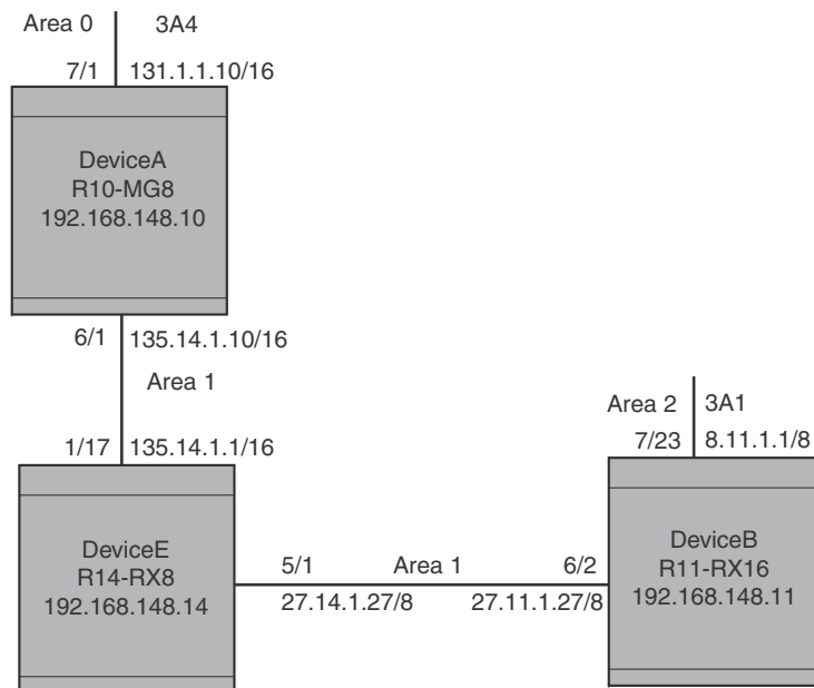
FIGURE 251 OSPF virtual neighbor and virtual link example
