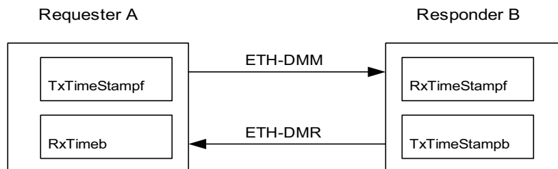
FIGURE 107 ETH-DM requester and responder.
