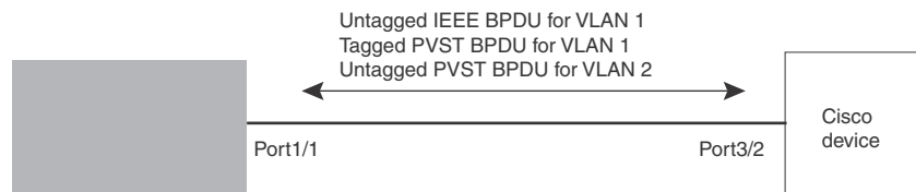
FIGURE 96 Port Native VLAN 2 for untagged BPDUs
