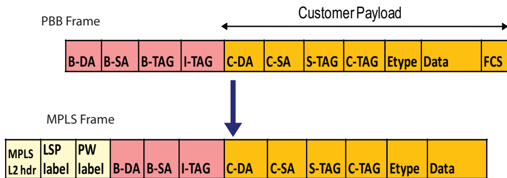
FIGURE 37 ISID mapping
