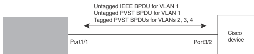
FIGURE 95 Default VLAN 1 for untagged BPDUs
