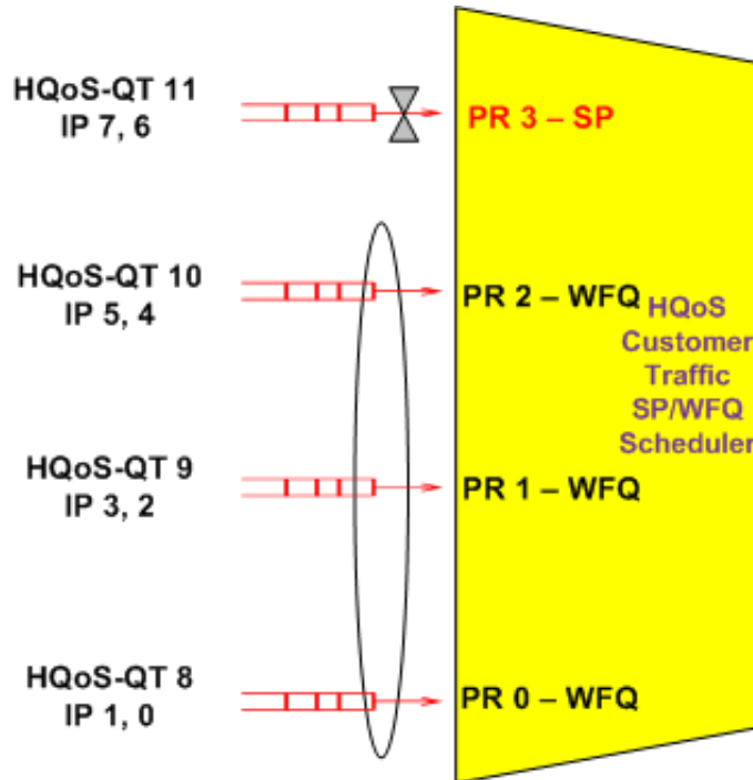
FIGURE 85 Mixed Strict Priority and Weighted Fair Queue
