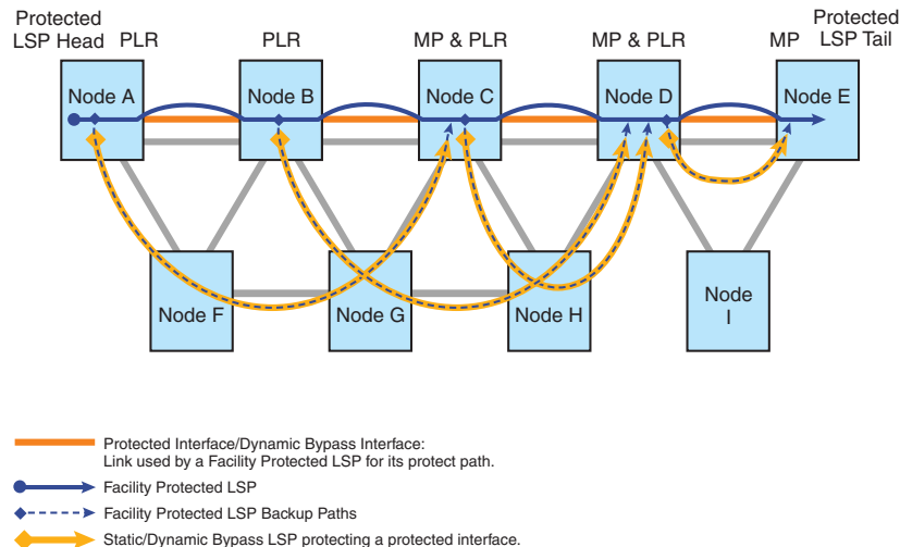
FIGURE 21 Protected dynamic bypass interface
