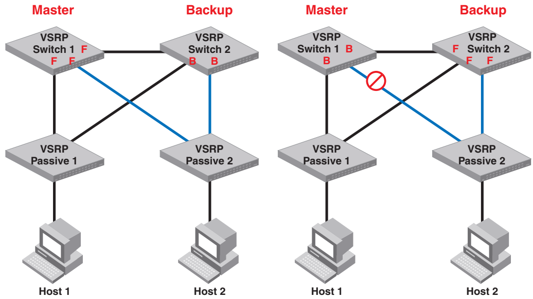
FIGURE 196 Black hole scenario 3
