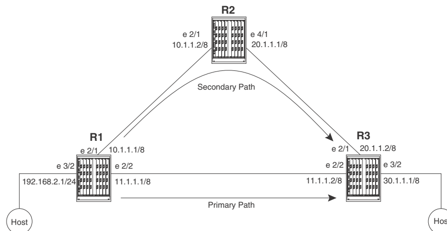
FIGURE 35 LSP configuration with primary and secondary paths
