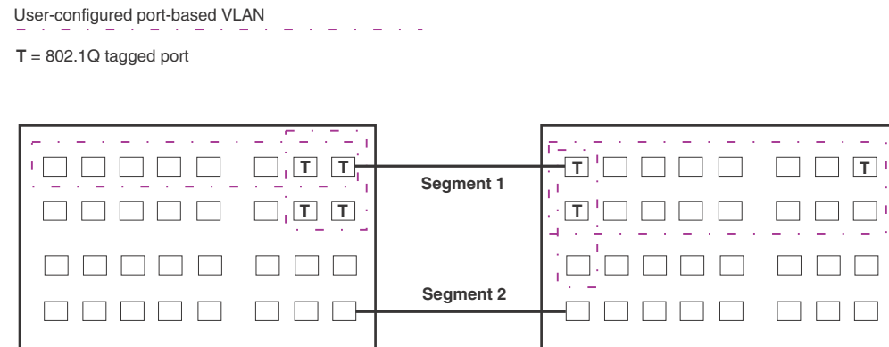
FIGURE 11 VLANs configured across multiple devices
