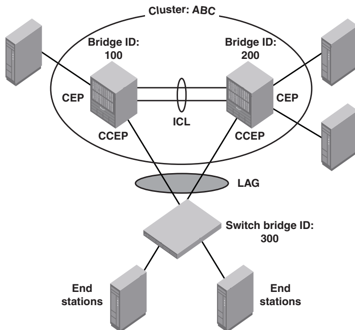
FIGURE 207 MCT Components
