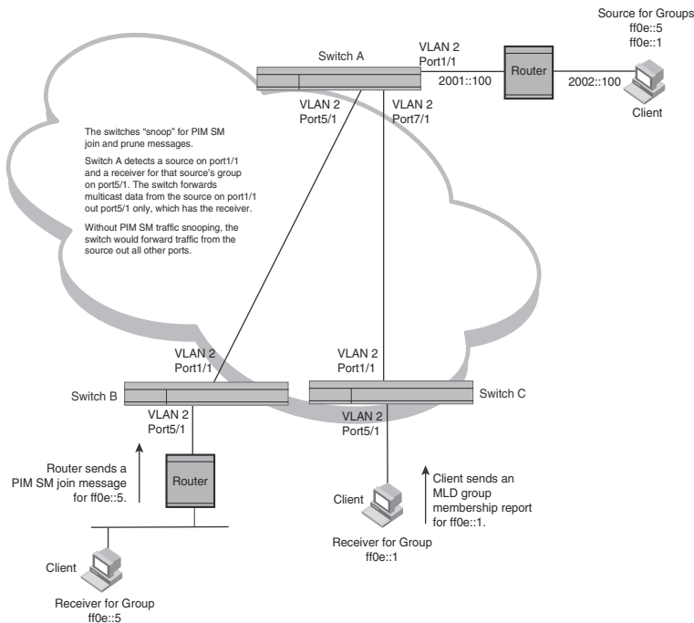
FIGURE 92 PIM-SM IPv6 traffic reduction in global Ethernet environment
