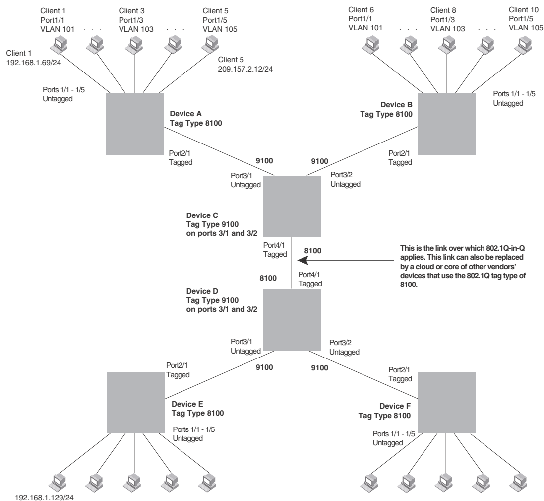
FIGURE 17 Example 802.1Q-in-Q configuration
