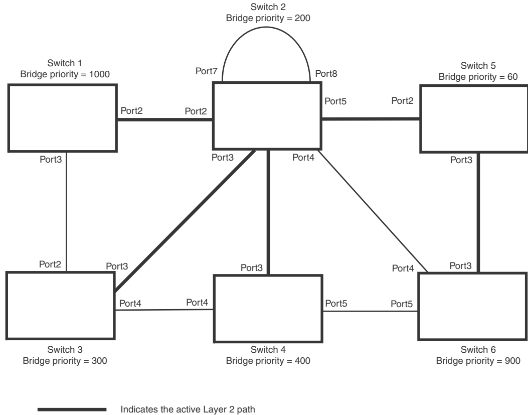
FIGURE 121 Active Layer 2 path in complex topology
