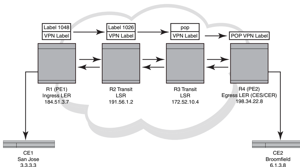
FIGURE 33 Traceroute in a Layer 3 VPN MPLS cloud
