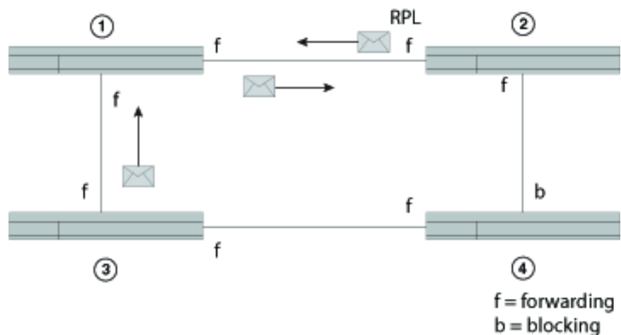
FIGURE 162 Initializing an ERP topology - IV
