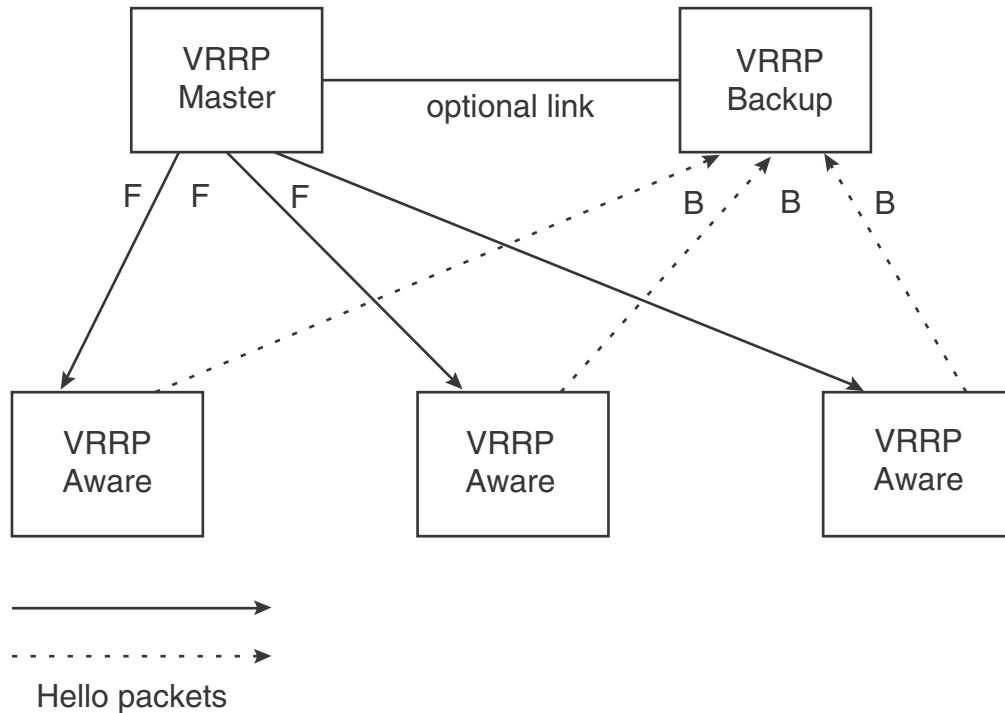
FIGURE 188 VSRP mesh – redundant paths for Layer 2 traffic
