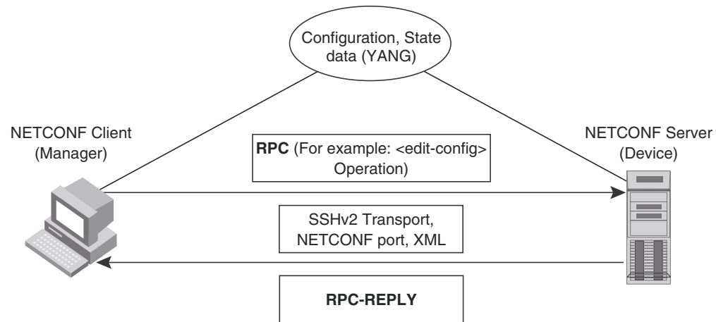
FIGURE 117 NETCONF communication
