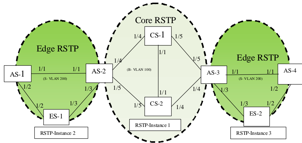
FIGURE 135 RSTP deployment in PB and PBB network
