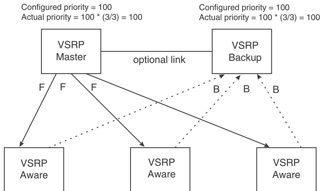
FIGURE 189 VSRP priority
