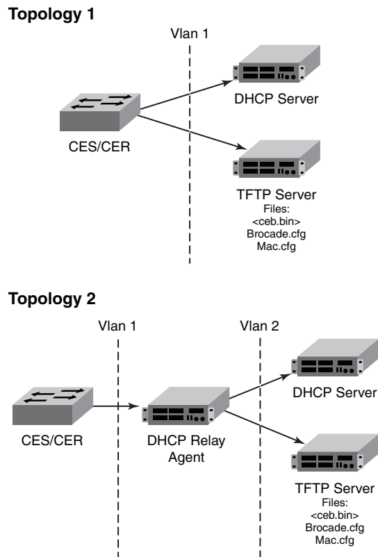
FIGURE 231 Zero Touch Provisioning
