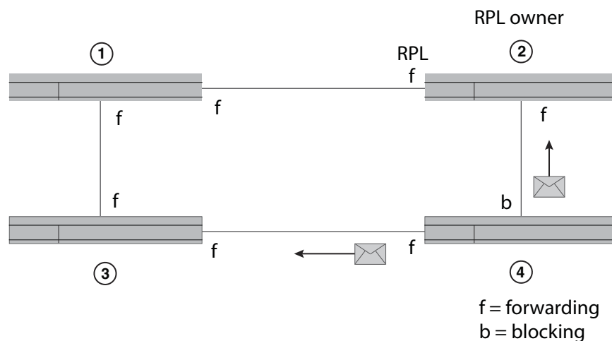
FIGURE 159 Initializing an ERN topology - I
