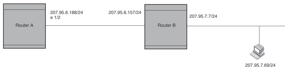
FIGURE 232 Example of a static route
