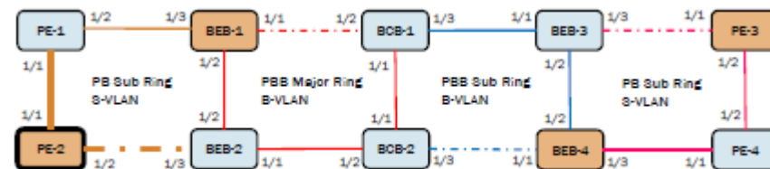
FIGURE 178 PB ring node sample configuration
