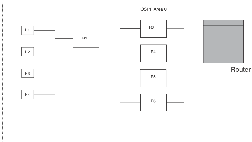
FIGURE 250 Example OSPF network with four equal-cost paths
