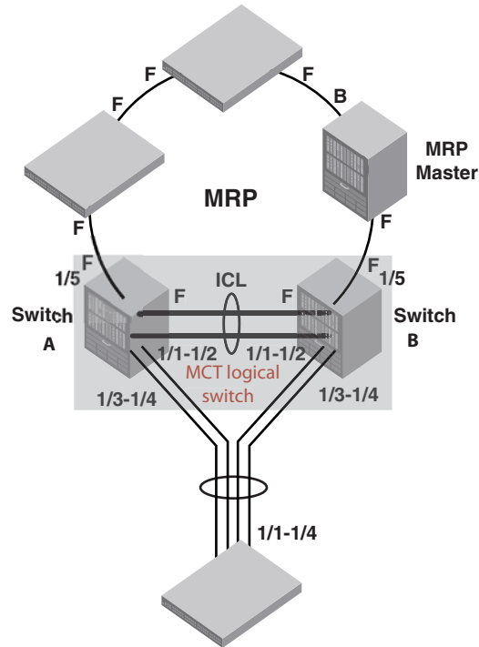
FIGURE 213 MRP integration with MCT
