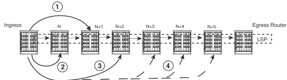
FIGURE 13 Fast reroute using one-to-one backup
