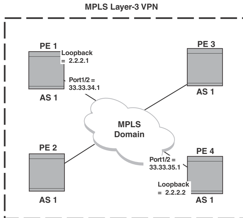
FIGURE 62 IBGP example
